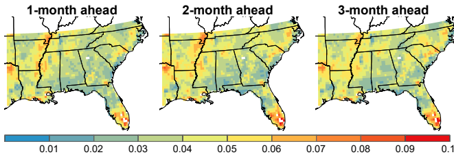
Figure 2. RMSE of the bias corrected 1-3 months ahead soil moisture forecasts based on the SMAP soil moisture observations
