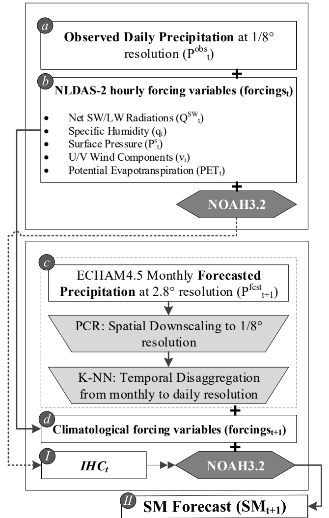
Figure 1. Soil moisture forecasting schematic. a) Observed precipitation forcings from Maurer et al. (2002) and b) observed non-precipitation land surface forcing fields from NLDAS-2 are implemented into the NOAH3.2 LSM to simulate I) the Initial Hydrologic Conditions (IHC) prior to each forecasting period. The IHCs are then used along with c) 1-3 month ahead ECHAM4.5 precipitation forecasts (spatially downscaled and temporally disaggregated, see section 2.1) and d) climatological forcings (i.e., mean of NLDAS-2 non-precipitation forcings over the period 1979-2010), in order to execute the NOAH3.2 LSM under a forecasting scheme and to develop II) 1-3 month ahead soil moisture forecasts.
