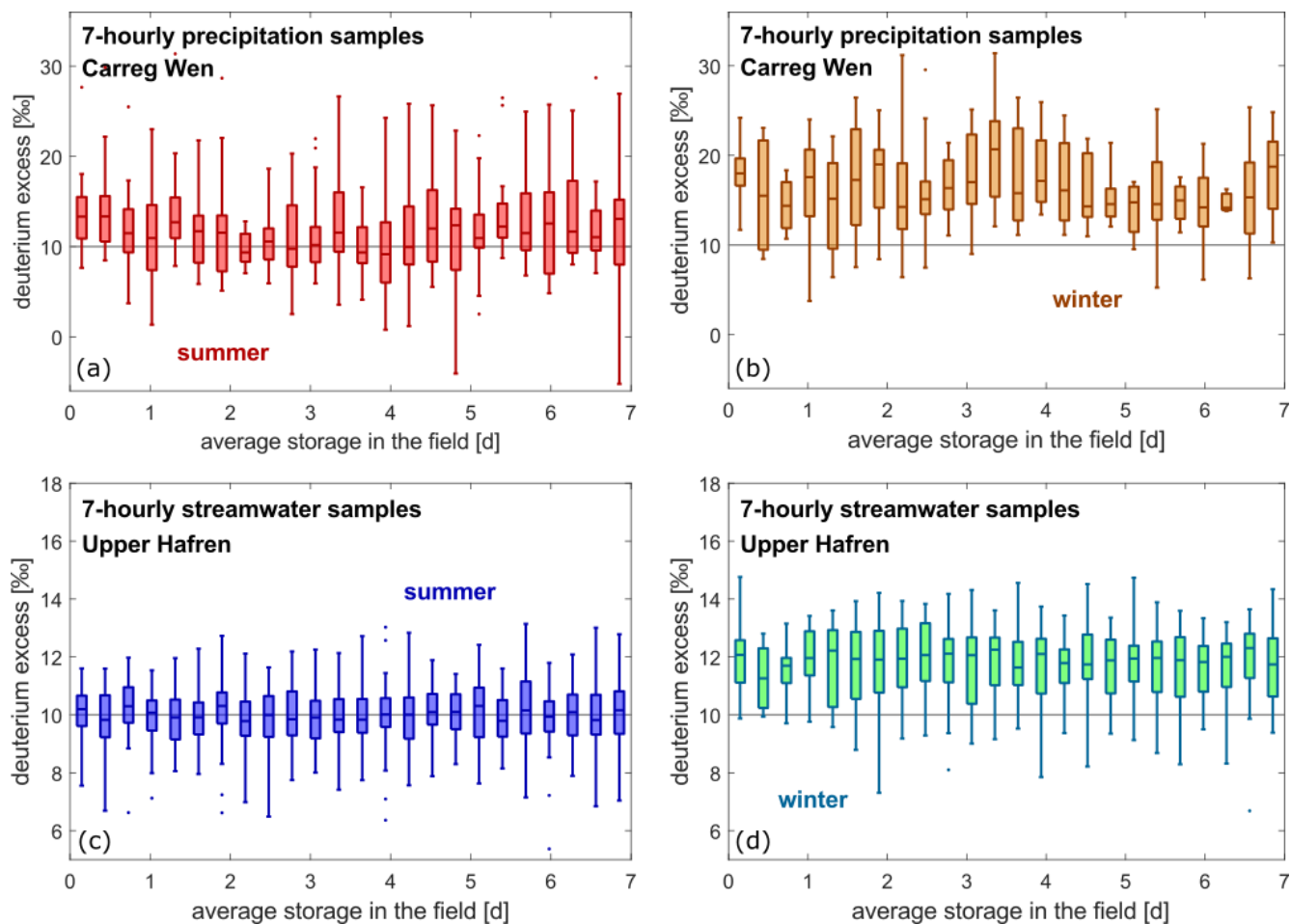
5 Figure 4: Variations in deuterium excess in 7-hourly samples as a function of the length of time that they were stored inside the field autosamplers. Boxplots are defined as described in Fig. 3. Axis scales differ between panels (a,b) and (c,d), reflecting the greater variability in precipitation deuterium excess. There is no systematic effect of storage duration on deuterium excess during either summer (May-October, panels a,c) or winter (November-April, panels b,d), indicating that any evaporative fractionation during storage was negligible. Deuterium excess in streamwater samples is systematically lower during summer, likely reflecting real-world seasonal variations in deuterium excess (see also Fig. 3).
