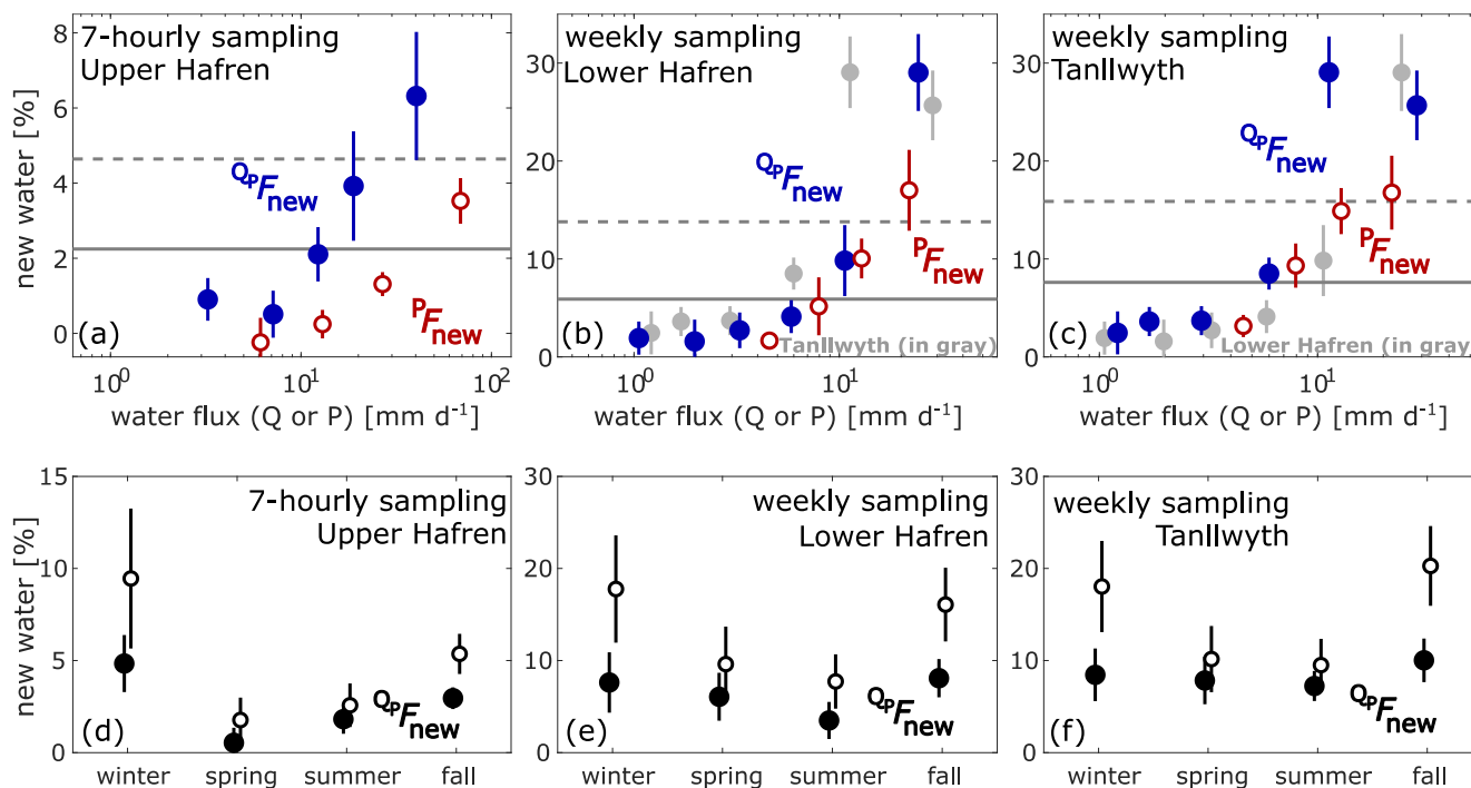
Figure 10: Event new water fractions ( Q_p F_{new} ) and new water fractions of precipitation ( P F_{new} ) for different discharge rates, precipitation rates, and seasons, calculated from time series of oxygen-18. Error bars indicate one standard error. In panels (a)-(c), solid circles indicate event new water fractions, plotted as functions of discharge rates, and open circles indicate new water fractions of precipitation, plotted as functions of precipitation rates. Gray markers in the background of panel (b) show event new water fractions from panel (c), and vice versa, to facilitate comparison between Lower Hafren and Tanllwyth. Event new water fractions are calculated for different percentiles of the discharge regime (in blue, 0–30, 30–60, 60–80, 80–90, and 90–100 for 7-hourly sampling, and 0–20, 20–40, 40–60, 60–80, 80–90, and 90–100 for weekly sampling; percentiles are calculated based only on discharge of time steps with precipitation, and precipitation thresholds were set to 0 \text{ mm h}^{-1} ). New water fractions of precipitation are calculated for different percentiles of precipitation rates above the precipitation threshold of 0.1 \text{ mm h}^{-1} (in red, 0–40, 40–60, 60–85, 85–100). Solid and dashed gray lines indicate unweighted and volume-weighted event new water fractions, respectively, across all discharge values. Panels (d)-(f) show event new water fractions, across all discharge values, determined separately for winter (December–February), spring (March–May), summer (June–August) and fall (September–November). Open and solid circles indicate volume-weighted and unweighted event new water fractions, respectively, in panels (d)-(f).
