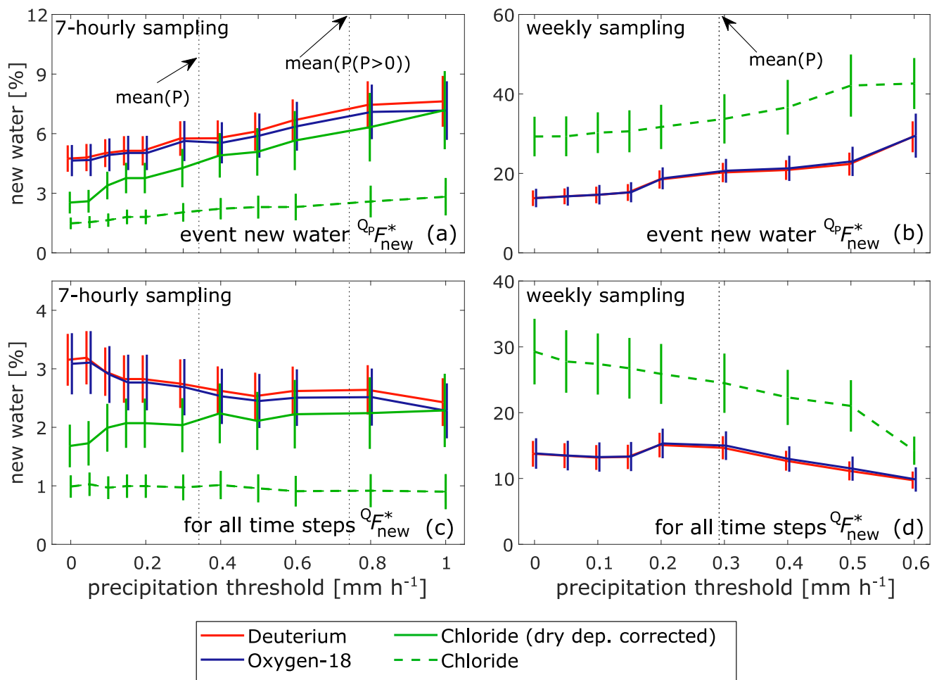
5 Figure 8: Effects of different precipitation thresholds on volume-weighted new water fractions for 7-hourly sampling at Upper Hafren (a, c) and weekly sampling at Lower Hafren (b, d). Error bars indicate one standard error. (a)-(b) show volume-weighted event new water fractions ( Q_p F_{new}^* ), which consider only time steps with precipitation. Higher precipitation thresholds lead to higher new water fractions in these panels, because time steps with low precipitation rates are usually associated with lower discharges. As these are excluded, fewer and fewer low-flow time steps are considered, increasing the relative importance of time steps with high discharge, which also tend to have higher new water fractions. Conversely, the precipitation threshold has less effect on volume-weighted new water fractions for all time steps ( Q F_{new}^* , c-d), because these include a factor that accounts for the fraction of days without precipitation. Precipitation thresholds have been slightly jittered for better visibility of the different tracers.
