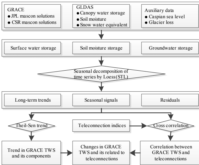
436 437 Figure 2: Methodology flow diagram of data processing in this study.
