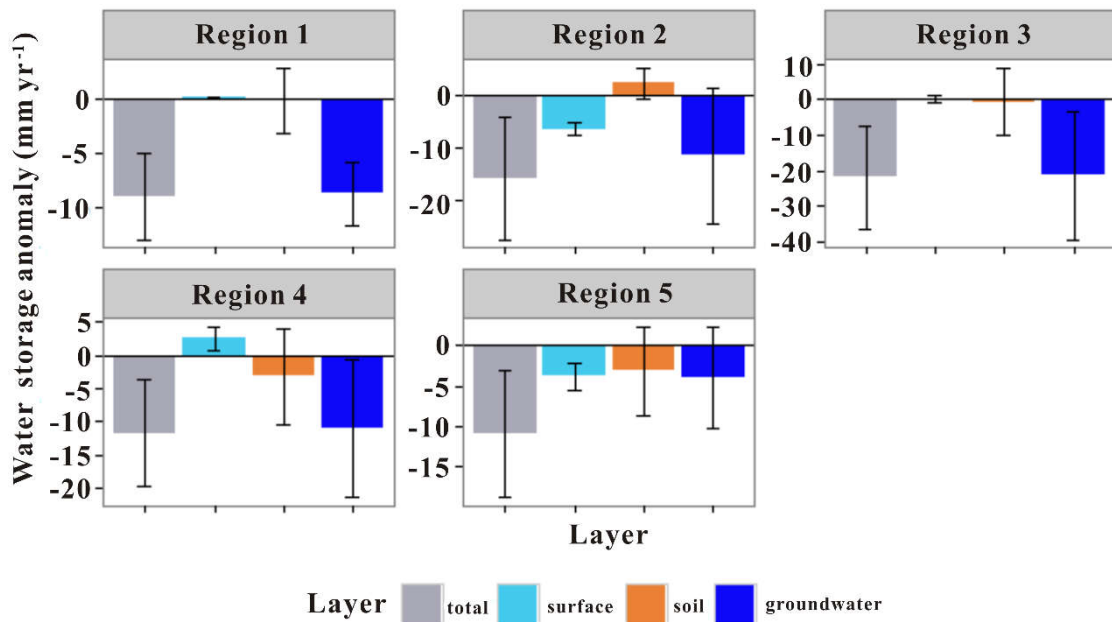
450 Figure 5: Contributions of different hydrological storages to TWS changes in five hotspots. Uncertainties represent the 95% 451 confidence intervals.
