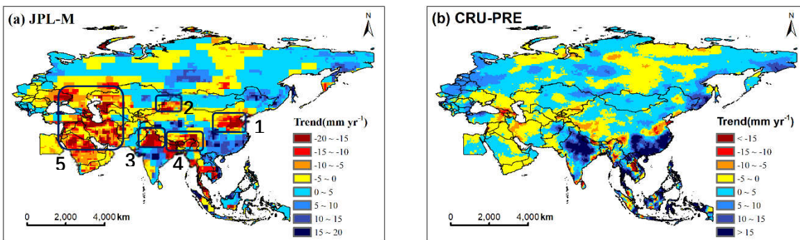
438 439 Figure 3: Spatiotemporal changes in TWS as obtained from GRACE (a) and precipitation as obtained from CRU (b) 440 across the Asian and Eastern European regions during 2002-2017. The trend is obtained from the removed seasonal 441 cycle time series.
