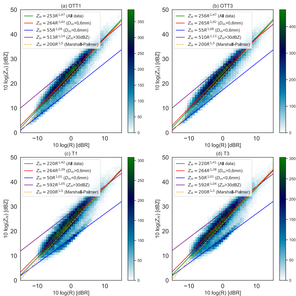
Figure 9: Horizontal reflectivity (in 10 \log_{10}(Z_H) [dBZ]) versus rain rate (in 10 \log_{10}(R) [dBR]) scatter plots for all co-located instruments (a to d). Power law relations are fitted separately for: all data, data meeting D_m > 0.6 mm (red curves), data meeting D_m < 0.6 mm (blue curves), data meeting Z_H > 30 dBZ (purple curves). The reference Marshall-Palmer relation is also shown.
