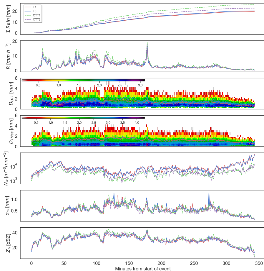
Figure 4: Rainfall Event #7 time-series of: (a) Cumulative rainfall amounts (mm); (b) Rainfall rate ( \text{mm h}^{-1} ); (c) Density distribution (log-scale) of drop size diameters for OTT1 (mm); (d) Density distribution (log-scale) of drop size diameters for T1 (mm); (e) Generalised intercept parameter ( \text{m}^{-3} \text{mm}^{-1} ); (f) Mass spectrum standard deviation (mm); and (g) Horizontal reflectivity (dBZ).
