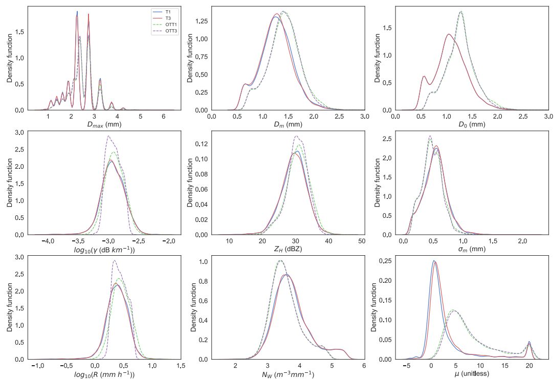
575 Figure A2. Frequency plots of the DSD parameters, based on distributions (not shown) of integrated variables ( D_{max} , D_m , D_0 , \gamma_H , Z_H , \sigma_m , R , N_W and \mu ) for the four instruments (T1, T3, OTT1, OTT3) for rainfall rates of 2 to 5 mm h -1 (6967 data points).
