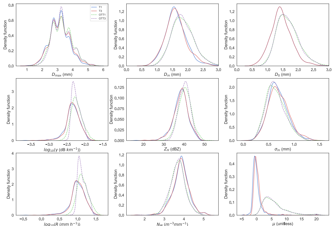
585 Figure A4. Frequency plots of the DSD parameters, based on distributions (not shown) of integrated variables ( D_{max} , D_m , D_0 , \gamma_H , Z_H , \sigma_m , R , N_W and \mu ) for the four instruments (T1, T3, OTT1, OTT3) for rainfall rates of 10 to 25 mm h -1 (753 data points).
