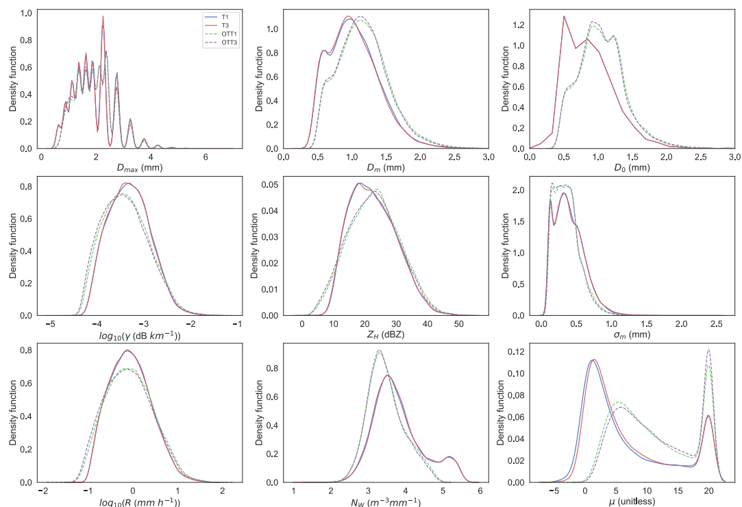
335 Figure 5: Density estimates of the DSD parameters ( D_{max} , D_m , D_0 , \gamma_H , Z_H , \sigma_m , R , N_W and \mu ) for the four instruments (T1, T3, OTT1, OTT3) for the full dataset.
