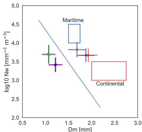
520 Figure 11: Average values of \log_{10} N_w versus D_m for the data presented in this study (OTT1 in blue, OTT3 in red, T1 in green, T3 in purple) and their standard deviations. The blue line represents the demarcation between stratiform rain (dot points) (below the line) and convective rain (cross) (above the line), and the rectangle cover the clusters of data corresponding to maritime-like and continental-like as defined by Bringi et al., (2003) and augmented by numbers of authors since.
