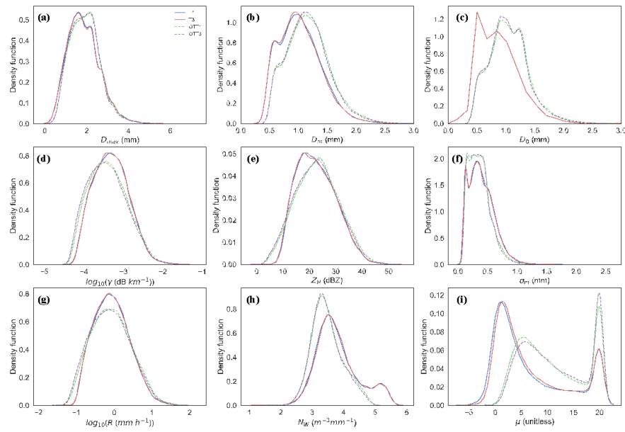
Figure 5: Density estimates of the DSD parameters ( D_{max} , D_m , D_0 , \gamma_H , Z_H , \sigma_m , R , N_k and \mu ) for the four instruments (T1, T3, OTT1, OTT3) for the full dataset.
