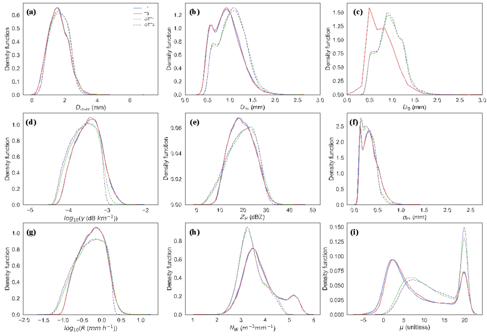
Figure A1. Frequency plots of the DSD parameters, based on distributions (not shown) of integrated variables ( D_{max} , D_m , D_0 , \gamma_H , Z_H , \sigma_m , R , N_W and \mu ) for the four instruments (T1, T3, OTT1, OTT3) for rainfall rates of 0.1 to 2 mm h -1 (29815 data points).
