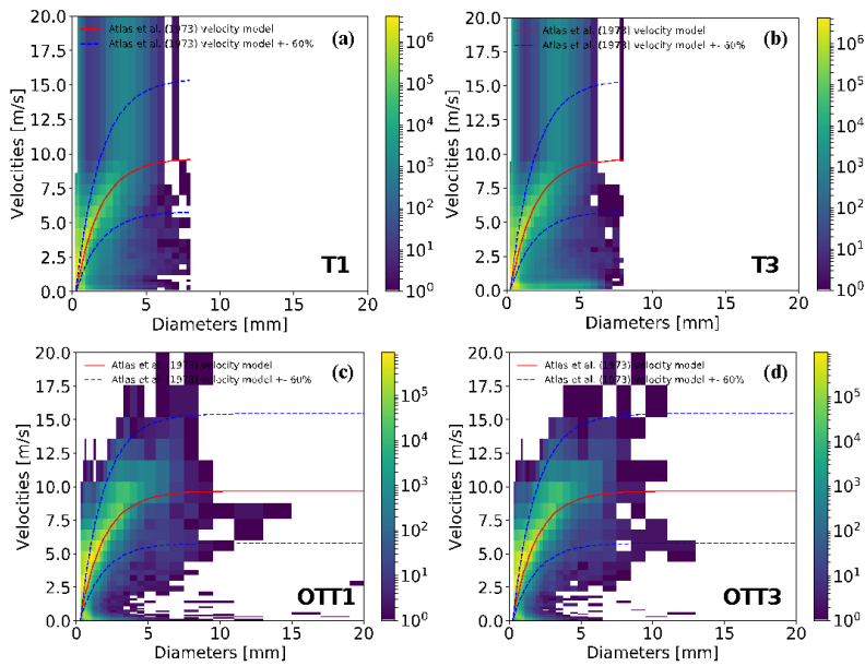
Figure 6: Particle velocity versus diameter density plots for the 2014-2017 period for the four instruments. The color scale indicates the number of particles for each bin (velocity and diameter). The velocity model of Atlas et al. (1973) is plotted in red together with its positive and negative deviations of 60%. This is used to filter outliers following Jaffrain and Berne (2011).
