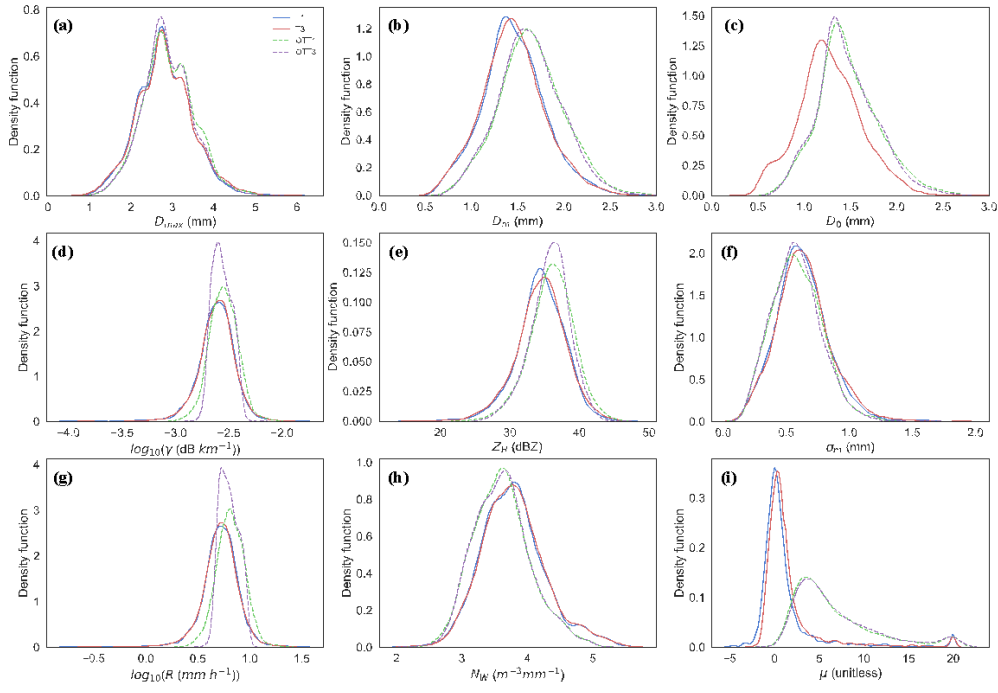
Figure A3. Frequency plots of the DSD parameters, based on distributions (not shown) of integrated variables ( D_{max} , D_m , D_0 , \gamma_H , Z_H , \sigma_w , R , N_W and \mu ) for the four instruments (T1, T3, OTT1, OTT3) for rainfall rates of 5 to 10 mm h -1 (2398 data points).
