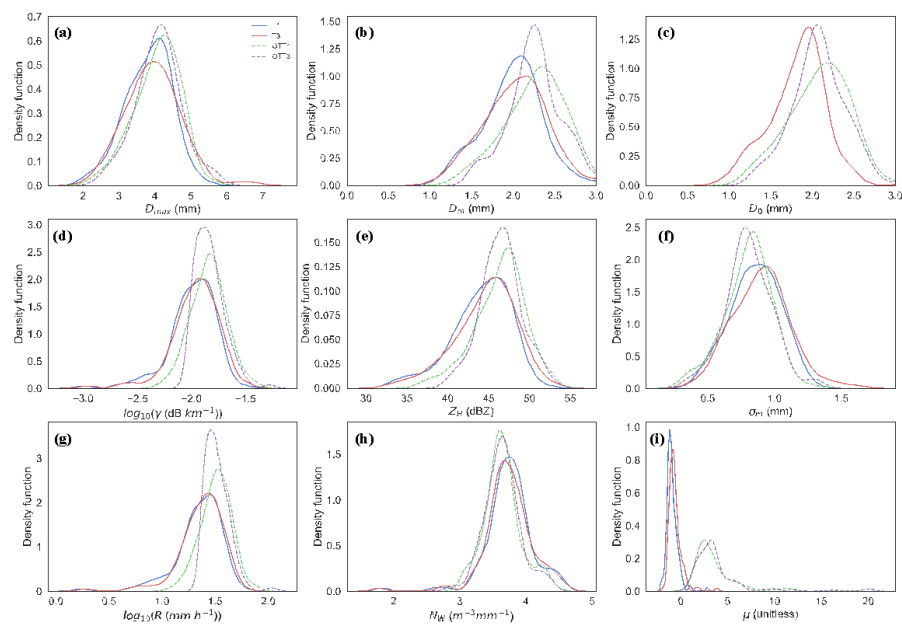
Figure 8: Frequency plots of the DSD parameters, based on distributions (not shown) of integrated variables ( D_{max} , D_m , D_0 , \gamma_H , Z_H , \sigma_m , R , N_W and \mu ) for the four instruments (T1, T3, OTT1, OTT3) for R > 25 \text{ mm h}^{-1} (129 data points).
