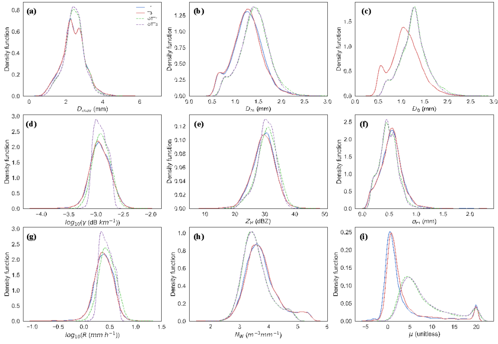
Figure A2. Frequency plots of the DSD parameters, based on distributions (not shown) of integrated variables ( D_{max} , D_m , D_0 , \gamma_H , Z_H , \sigma_H , R , N_W and \mu ) for the four instruments (T1, T3, OTT1, OTT3) for rainfall rates of 2 to 5 mm h -1 (6967 data points).
