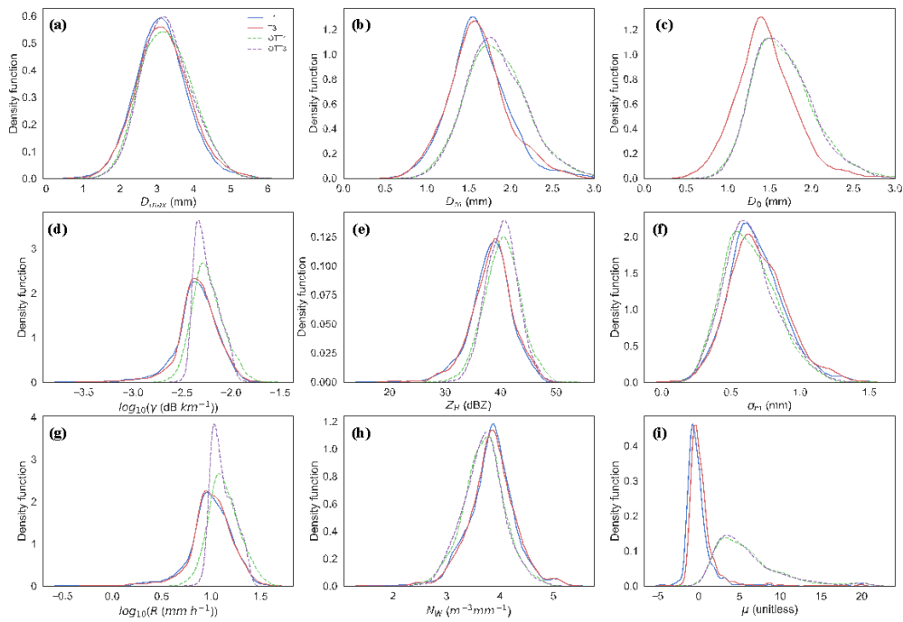
Figure A4. Frequency plots of the DSD parameters, based on distributions (not shown) of integrated variables ( D_{max} , D_m , D_0 , \gamma_H , Z_H , \sigma_n , R , N_W and \mu ) for the four instruments (T1, T3, OTT1, OTT3) for rainfall rates of 10 to 25 mm h -1 (753 data points).
