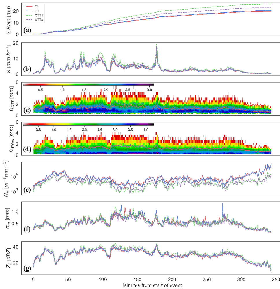
Figure 4: Rainfall Event #7 time-series (the event started on 24 th September 2014 at 9:09 AEDT) of: (a) Cumulative rainfall amounts (mm); (b) Rainfall rate ( \text{mm h}^{-1} ); (c) Density distribution (log-scale) of drop size diameters for OTT1 (mm); blue line is OTT1 D_m (mm) and red line is OTT3 D_m (mm); (d) Density distribution (log-scale) of drop size diameters for T1 (mm); blue line is OTT1 D_m (mm) and red line is OTT3 D_m (mm); (e) Generalised intercept parameter ( \text{m}^{-3} \text{mm}^{-1} ); (f) Mass spectrum standard deviation (mm); and (g) Horizontal reflectivity (dBZ).
