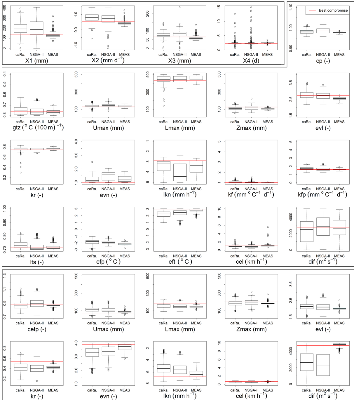
Figure 10. Calibrated parameter distributions for the sets on the Pareto front (y limits are the calibration bounds, except for X1 to X4) with caRamel, NSGA-II and MEAS for the three hydrological case studies: Blue River (first block of four parameters), Durance River (second block of 16 parameters) and Tarn River (third block of 10 parameters). Parameter values from the “best compromise” set are displayed in red. TS3
