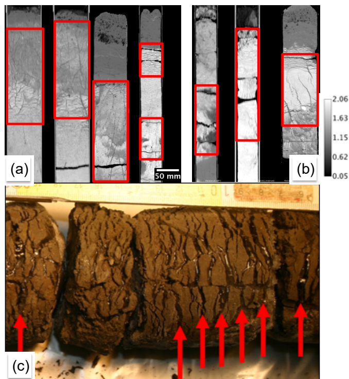
5 Figure 12. Vertical cross sections of X-ray CT scans of the top 40 cm of cores from (a) low-centered polygons and (b) high-centered polygons. The CT scans show the density distribution from low (dark) to high (white) with a calibration bar shown in \text{g}/\text{cm}^3 . Red boxes indicate patterns of vertical and horizontal density contrasts. Frozen core sampled from saturated tundra (c) is analogous to a low-centered polygon. Red arrows indicate prominent ice lenses. Ice lenses are formed at freeze-up when the soil is sufficiently saturated. Notice that most ice lenses are horizontal relative to ground surface. Photo credit: Vladimir Romanovsky.
