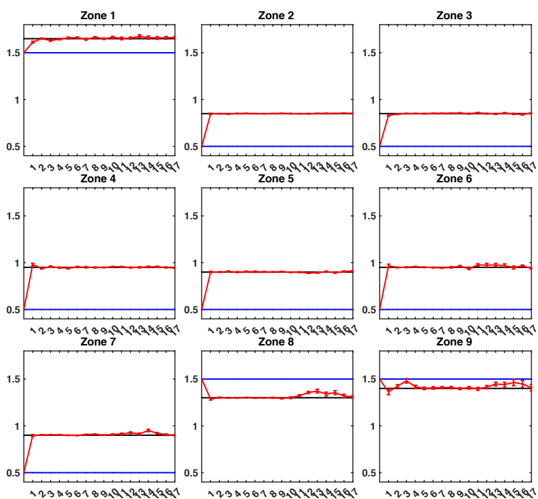
Figure 7. Control variables assimilation results for the PE1 experiment: evolution of the ensemble-averaged analysis control variable (red line) for each zone (one zone per subplot) with respect to the assimilation cycle and compared to the corresponding true value (black line) and the openloop value (blue line).
