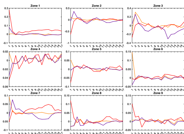
Figure A1. Evolution of the EnKF innovations (" y_k^{o,[l]} - \mathcal{H}_k(x_k^{b,[l]}) ") term in Eq. 12) with respect to the assimilation cycle for PE1 (red line), PE2 (orange line) and PE3 (purple line). For each zone (one zone per subplot), the displayed innovation is the averaged of all the innovations in the corresponding zones.
