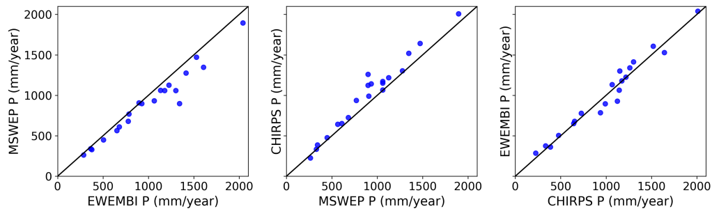
Fig. 1. Figure 5: Comparison of EWEMBI, MSWEP, CHIRPS precipitation products on their prediction of mean P across the basins
