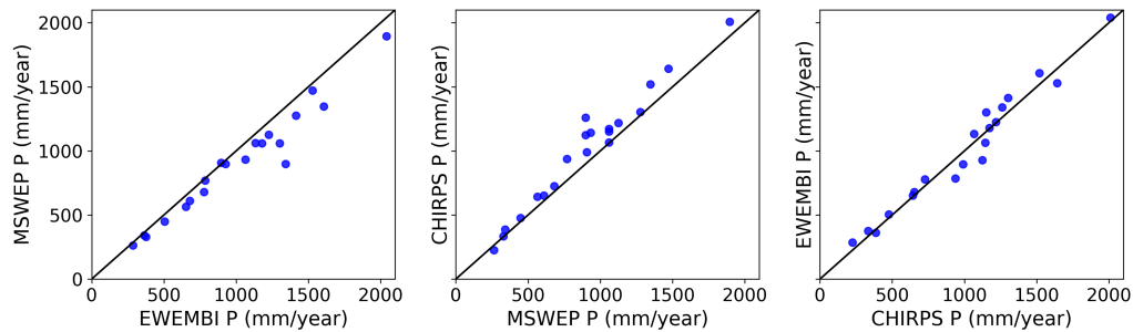
Fig. 6. Comparison of EWEMBI, CHIRPS and MSWEP precipitation products on their prediction of mean P across the basins
