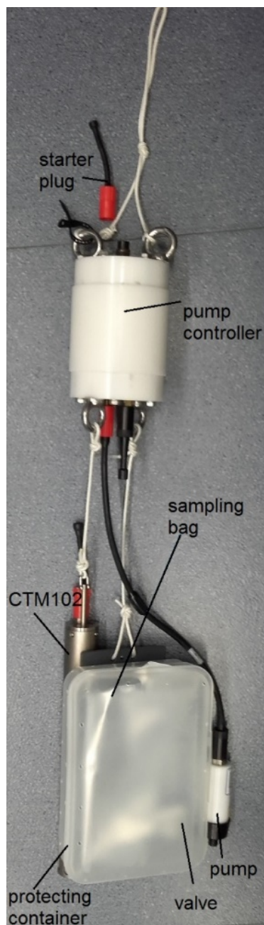
Figure 2: Gas sampling arrangement as used in Lake Kivu with pump controller, submersible pump, and protection housing for the sampling bag; a small CTD-probe was connected to record depth, electrical conductivity and temperature and started synchronously with the pump controller using a starter plug.
