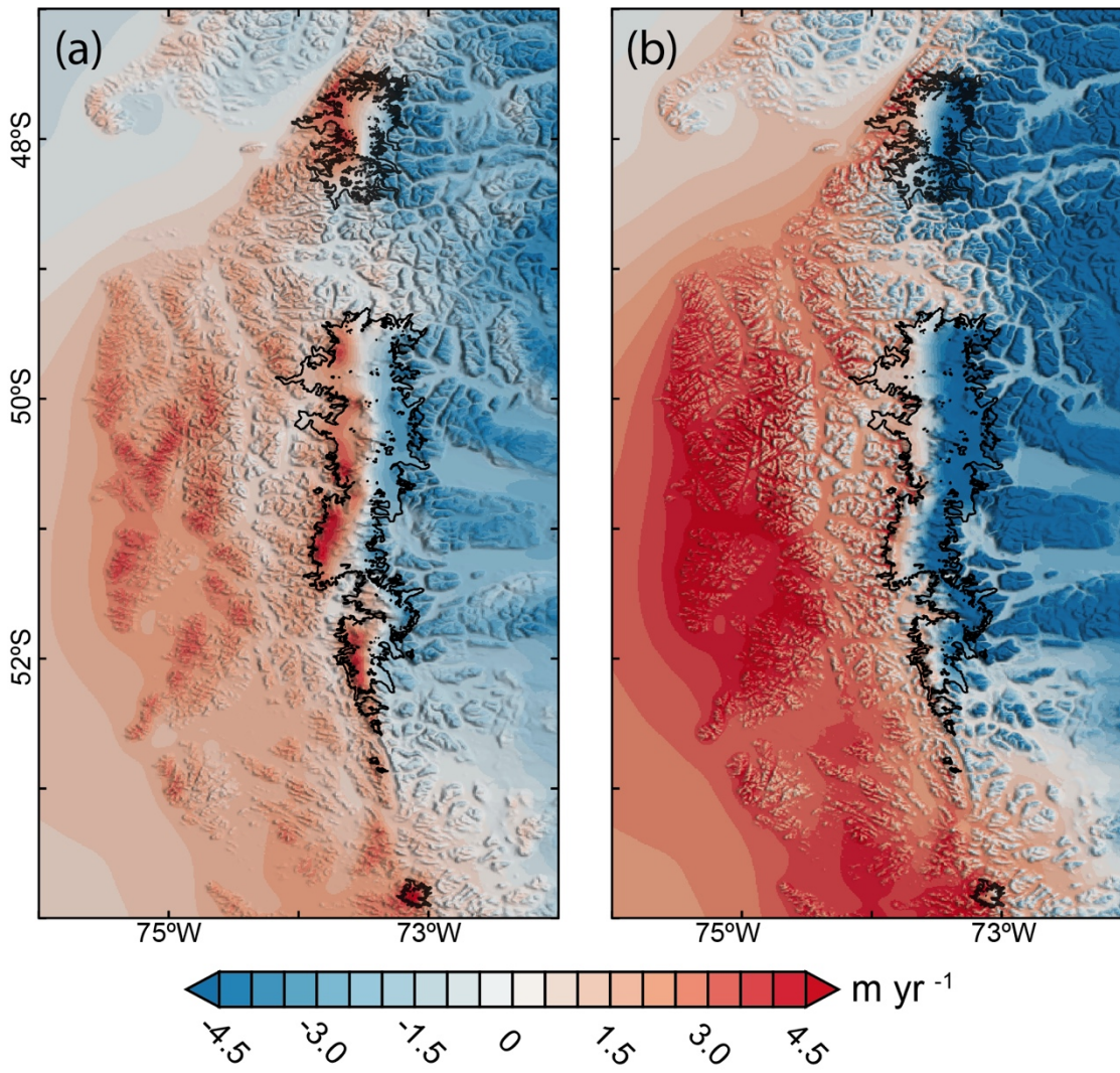
Figure 4: Differences between the OPM ensemble experiments and the DR-scaling approach. Panel (a) shows the differences in \text{m yr}^{-1} between the OPM 0.45 and DRS 0.45 experiment. Similarly, panel (b) shows the differences between OPM 0.60 the DRS 0.60 .
