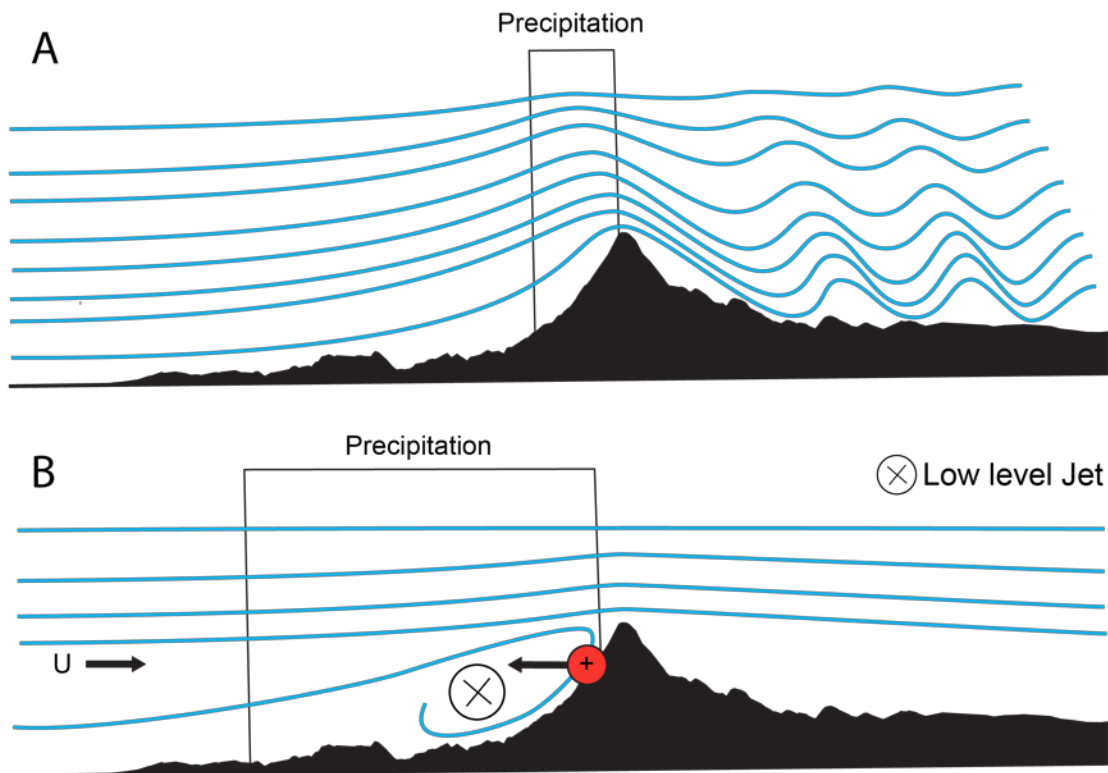
5 Figure 7: Schematic illustration of the interaction between the atmospheric air flow and the Andes. (A) Linear mountain flow response ( \hat{H} < 1 ) leads to strong uplift and precipitation along the west slopes. (B) The air flow is blocked by the topography ( \hat{H} \geq 1 ) and the resulting pressure gradient (indicated by the red circle) at the west slope slows down the upstream flow. The imbalance between the large-scale pressure gradient and Coriolis-force leads to a northerly low-level jet, which reduces and shifts the uplift motions upstream. This mechanism enhances precipitation in the Pre-Cordillera range, while reducing precipitation at the west slopes of the Andes.
