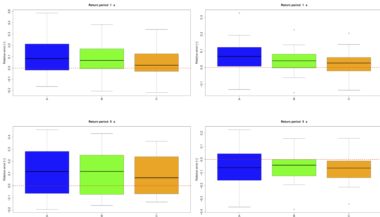
Fig. 7: Mean relative errors of extreme values of the disaggregated time series for all stations (the dashed line represents an error of 0). Results are shown for durations of 5 min (left) and 1 h (right) and for return periods of 1 year (top) and 5 years (bottom).
