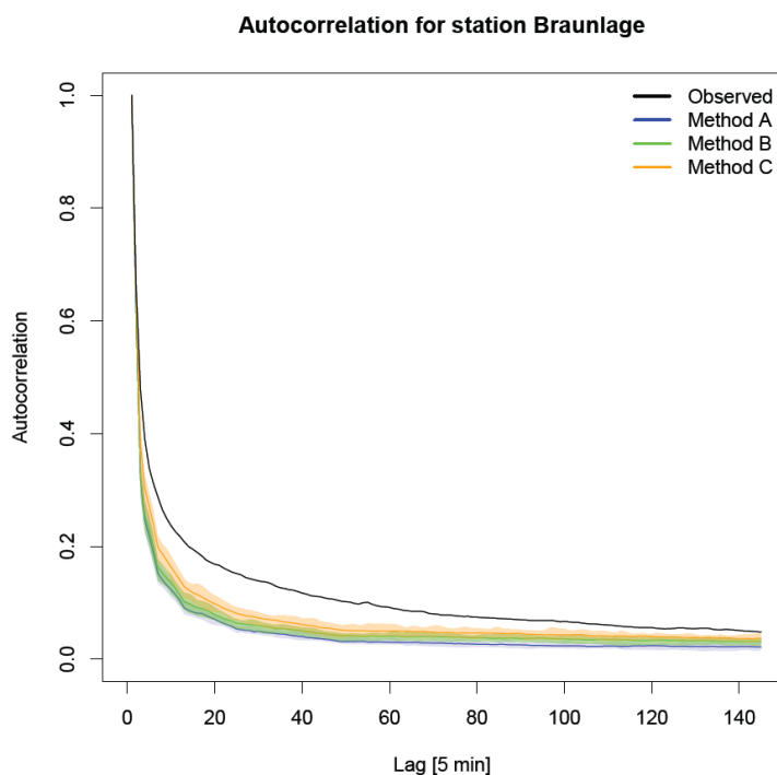
Fig. 5: Autocorrelation of observed and disaggregated time series using the standard approach for each method with no modification regarding too small rainfall intensities. The range for each method results from 30 realisations, the solid line represents the median.
