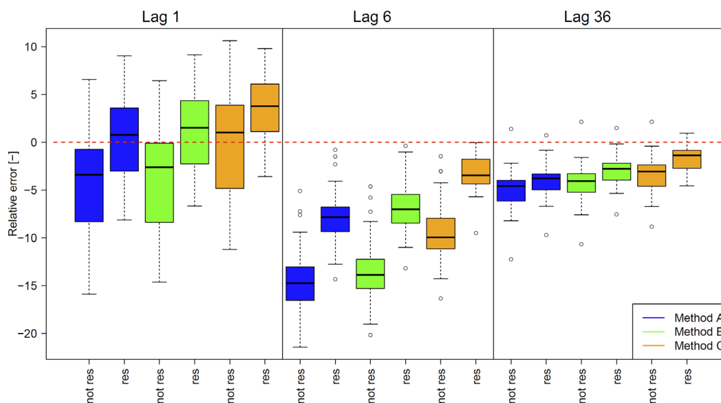
Fig. 8: Deviations of autocorrelation from disaggregated to observed time series before and after the resampling as relative error for lags 1, 6 and 36. All results are based on the MMD approach. The red dashed line indicates a rE=0 , results for the resampled time series are labelled with ‘res’.
