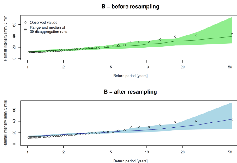
Fig. 9 Extreme rainfall values for D=5 min for station Osnabrück based on 30 disaggregation realisations with method B before (upper part) and after (lower part) the resampling
