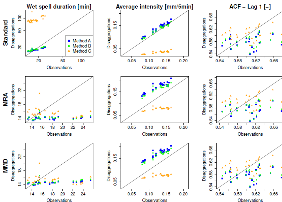
15 Fig. 4: Rainfall characteristics of observed and disaggregated time series as x-y plots for all 24 stations (note the different scales for wet spell duration)
