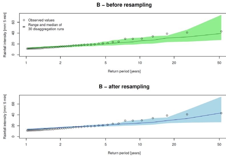
Fig. 11 Extreme rainfall values for D=5 min for station Osnabrück based on 30 disaggregation realisations with method B before (upper part) and after (lower part) the resampling
