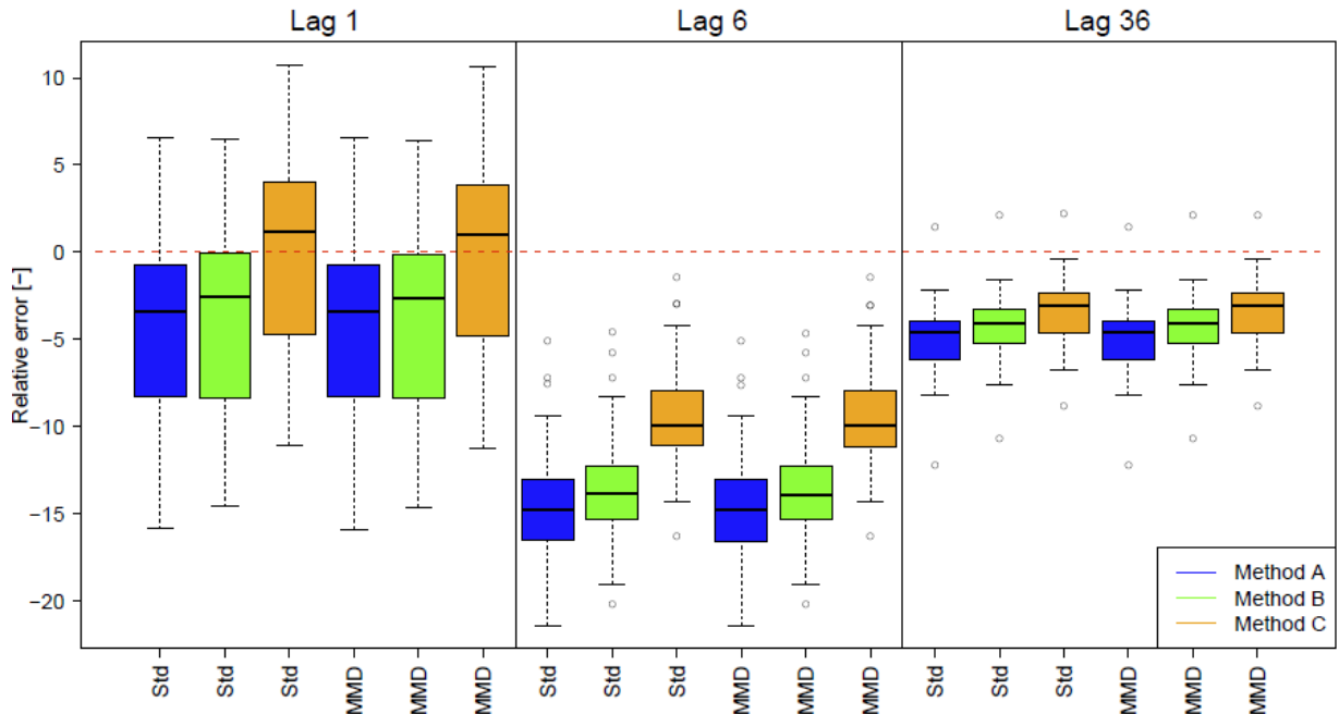
Fig. 8: Deviations of autocorrelation from disaggregated to observed time series as relative error for lags 1, 6 and 36. The red dashed line indicates a rE=0 (Std is used as abbreviation for Standard)
