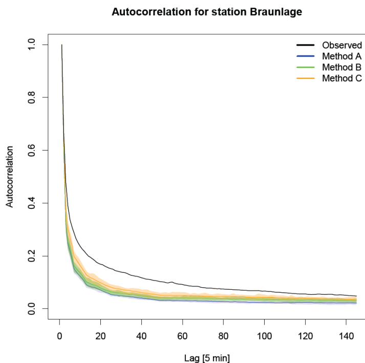
Fig. 7: Autocorrelation of observed and disaggregated time series using the standard approach for each method with no modification regarding too small rainfall intensities. The range for each method results from 30 realisations, the solid line represents the median.
