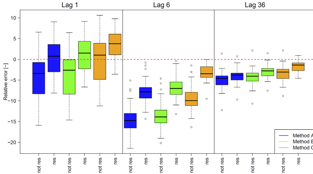
Fig. 10: Deviations of autocorrelation from disaggregated to observed time series before and after the resampling as relative error for lags 1, 6 and 36. All results are based on the MMD approach. The red dashed line indicates a rE=0 , results for the resampled time series are labelled with ‘res’.
