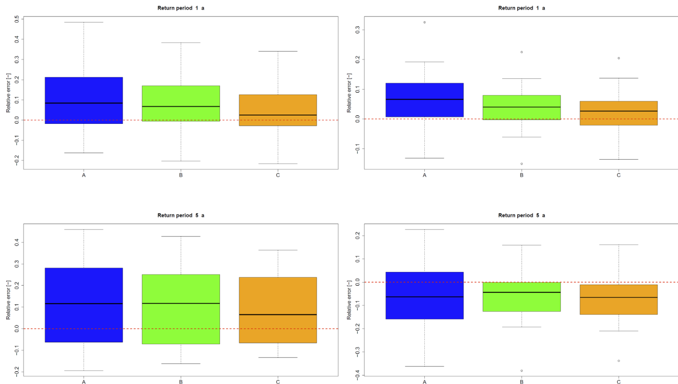
Fig. 9: Mean relative errors of extreme values of the disaggregated time series for all stations (the dashed line represents an error of 0). Results are shown for durations of 5 min (left) and 1 h (right) and for return periods of 1 year (top) and 5 years (bottom).
