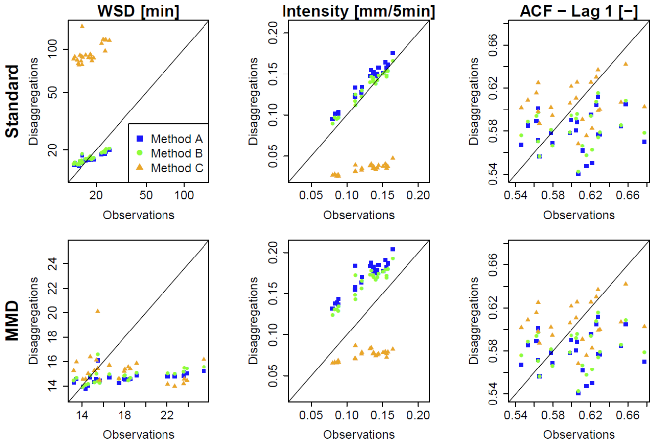
15 Fig. 7: Rainfall characteristics of observed and disaggregated time series as x-y plots for all 24 stations (WSD=wet spell duration, ACF=autocorrelation function; note the different scales for wet spell duration)
