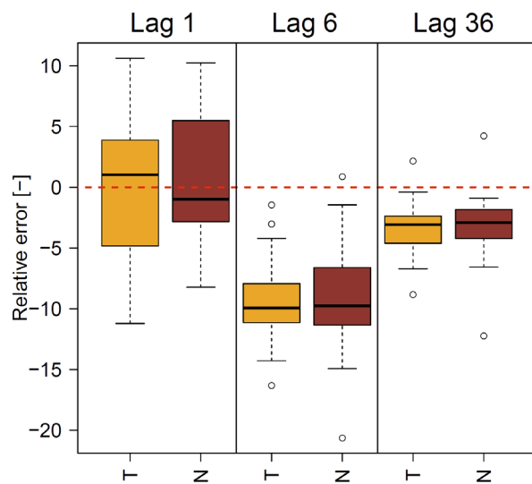
Fig. S4.1: Deviations of autocorrelation from disaggregated to observed time series for method C as rE for lags 1, 6 and 36 in dependence of the location used for parameter estimation. The red dashed line indicates a rE=0 (Std is used as abbreviation for Standard)
