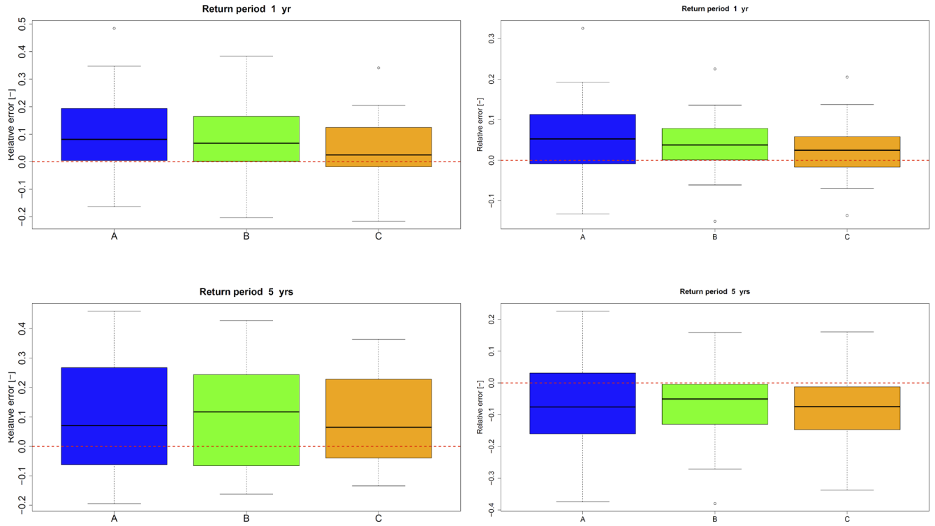
Fig. 10: Mean relative errors of extreme values of the disaggregated time series for all stations (the dashed line represents an error of 0). Results are shown for durations of 5 min (left) and 1 h (right) and for return periods of 1 year (top) and 5 years (bottom).
