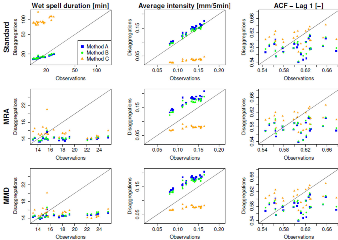
Fig. 5: Rainfall characteristics of observed and disaggregated time series as x-y plots for all 24 stations (note the different scales for wet spell duration)
