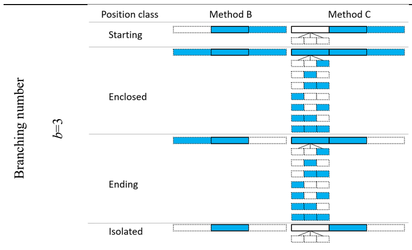
20 Fig. 3: Comparison of position classes definition for methods A, B and C. For method A, no position classes differentiation is applied for b=3 . The dashed boxes indicate the time steps, which are analysed regarding their wetness state for the definition of the position class. Blue boxes indicate a wet time step, white boxes a dry time step.
