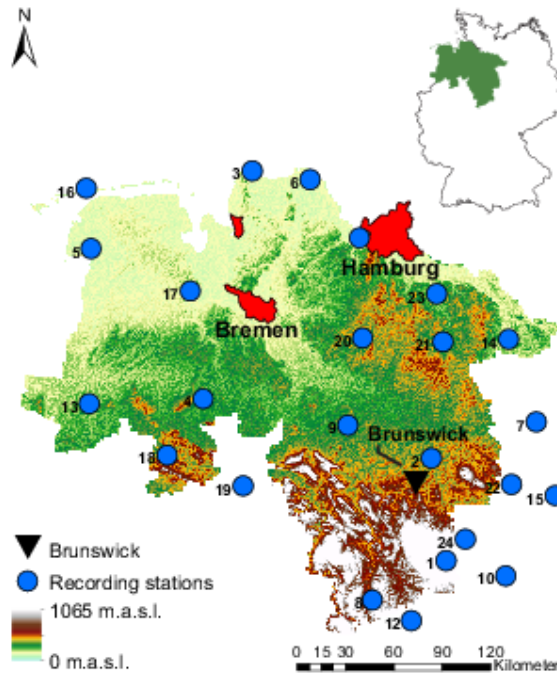
5 Fig. 1: Study area of Lower Saxony (and its location in Germany) with 24 recording stations.
