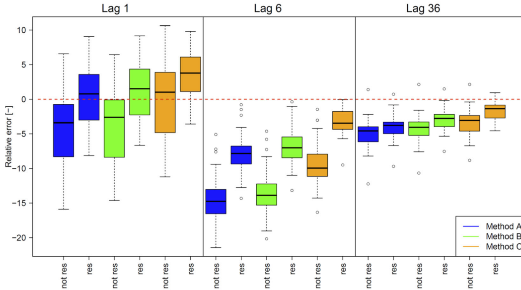
Fig. 9: Deviations of autocorrelation from disaggregated to observed time series before and after the resampling as relative error for lags 1, 6 and 36. All results are based on the MMD approach. The red dashed line indicates a rE=0 , results for the resampled time series are labelled with ‘res’.
