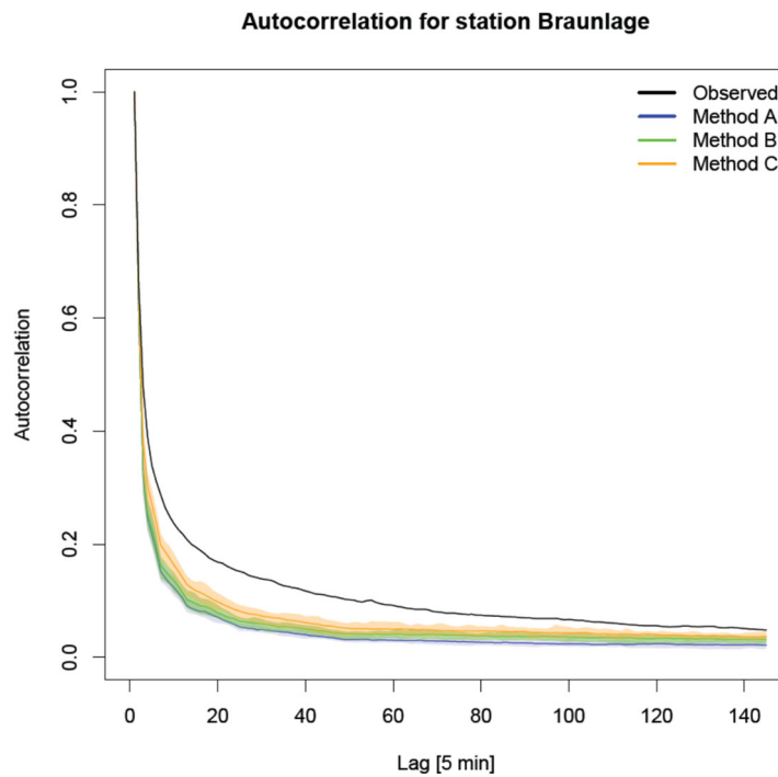
15 Fig. 6: Autocorrelation of observed and disaggregated time series using the standard approach for each method with no modification regarding too small rainfall intensities. The range for each method results from 30 realisations, the solid line represents the median.
