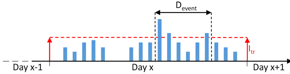
Fig. 4: Scheme for extreme rainfall event definition
