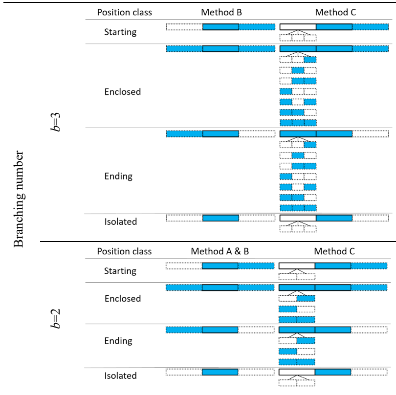
Fig. 3: Comparison of position classes definition for methods A, B and C. For method A, no position classes differentiation is applied for b=3 . The dashed boxes indicate the time steps, which are analysed regarding their wetness state for the definition of the position class. Blue boxes indicate a wet time step, white boxes a dry time step.
