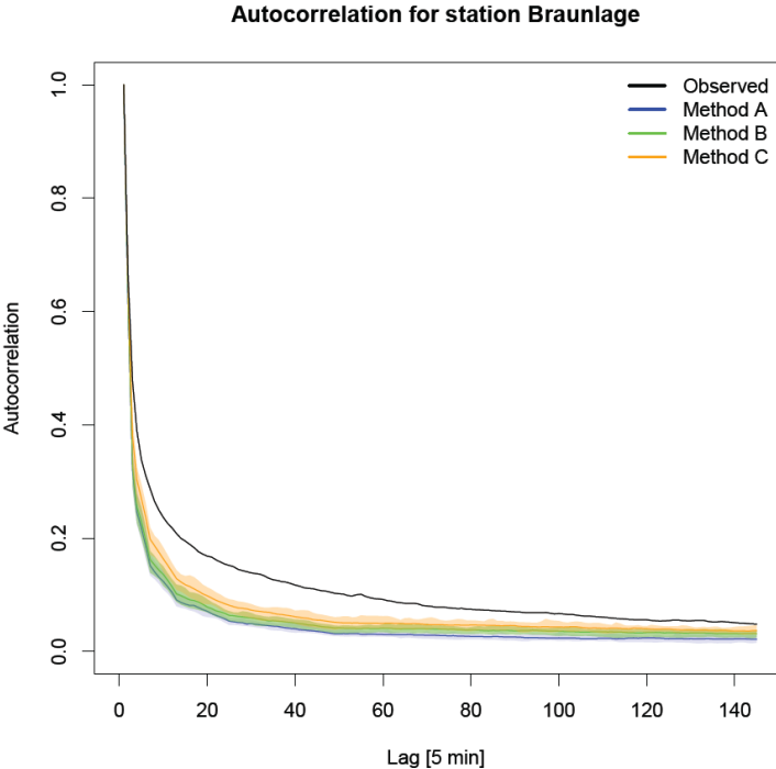
5 Fig. 6: Autocorrelation of observed and disaggregated time series using the standard approach for each method with no modification regarding too small rainfall intensities. The range for each method results from 30 realisations, the solid line represents the median.
