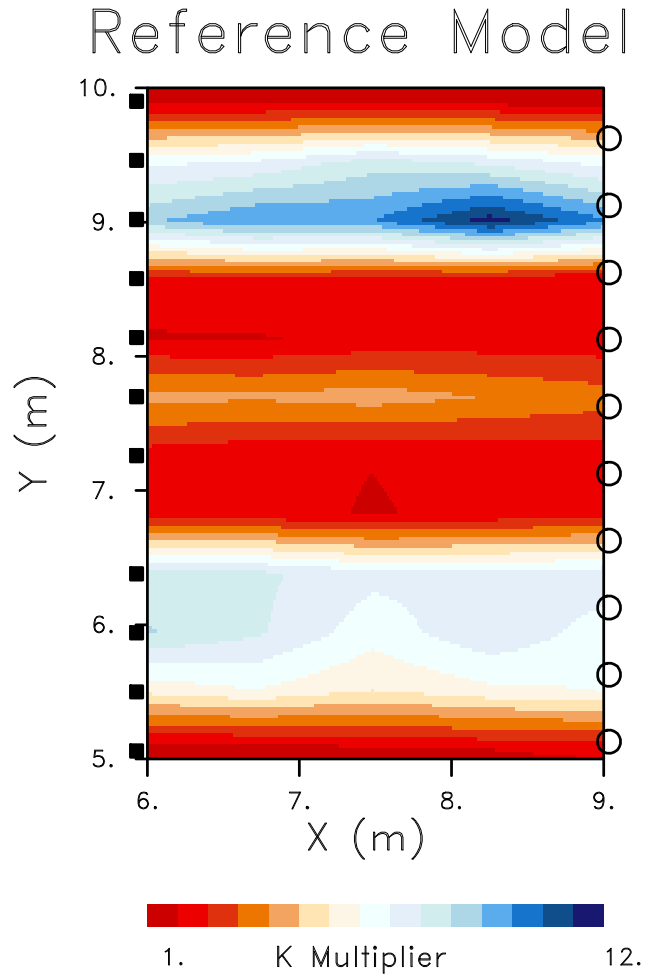
Figure 2. Reference model for the crosswell test example. A cross-section through the permeability model representing the crosswell plane. The crosswell configuration, for imaging flow properties between two boreholes, consists of pressure sources in the two wells (filled squares and open circles) transmitting transient pulses to receivers (open circles) in an adjacent well. The source-receiver geometry mimics that of the field experiment conducted in Widen, Switzerland. The color scale varies linearly between permeability multipliers from 1 to 12.
