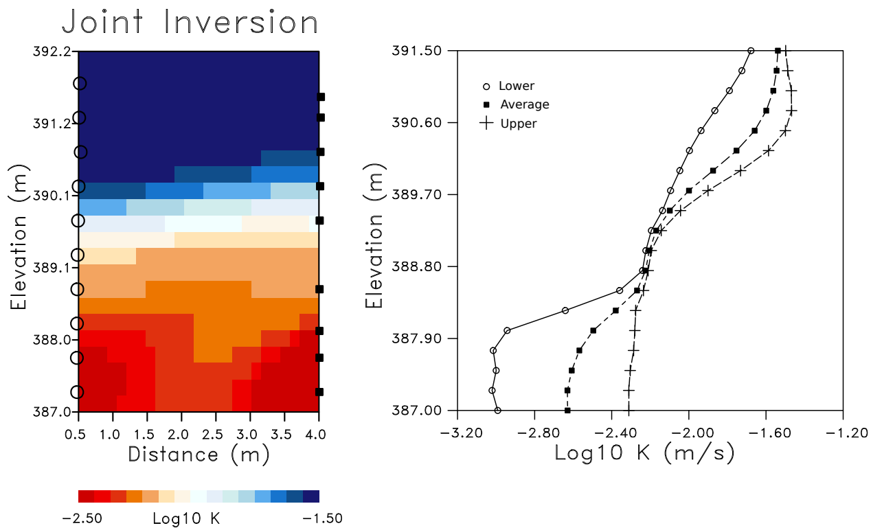
Figure 15. (Left panel) The portion of the inversion results of Lochbühler et al. [2013] that corresponds to our inversion domain. Their joint inversion includes ground-penetrating radar travel times as well as travel times and amplitudes from crosswell slug tests. (Right panel) The highest and lowest permeabilities at each depth in the inversion domain, plotted along with the average permeability as a function of elevation.
