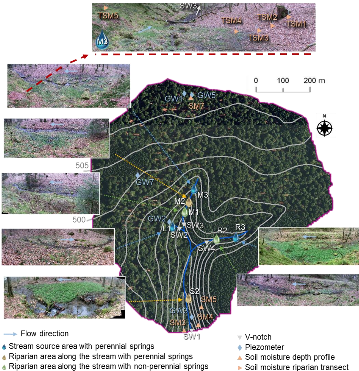
15 Figure 1: Weierbach catchment with the locations of the installed v-notch weirs for measuring discharge (SW1-SW4), piezometers for measuring groundwater levels (GW1-GW3, GW5, GW7), soil moisture sensors for measuring soil moisture in different depth profiles (SM3-SM5, SM7) and a riparian transect (TSM1-TSM5), and the seven investigated riparian areas along the left (L1), middle (M1-M3), and right (R2, R3) tributary and the central stream (S2). Orthophoto of the catchment: Administration du Cadastre et de la Topographie 2010 (geoportail.lu).
