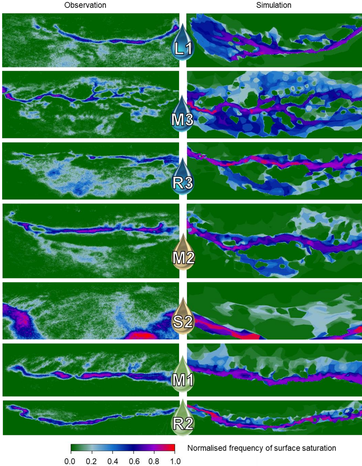
10 Figure 7: Observed (left) and simulated (right) frequencies of surface saturation in the seven investigated riparian areas along the left (L1), middle (M1-M3), and right (R2, R3) tributary, and the central stream (S2) (cf. Fig. 1). The maps were created by first counting how often the individual pixels were classified as saturated in the individual panoramic images and second normalizing the resulting frequency numbers by the total number of images analysed for the respective area.
