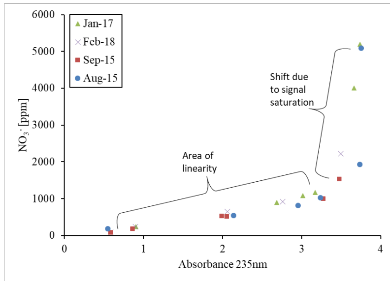
Figure S5 - Shift in measuring high concentrations at 235nm: Open crop field nitrate concentration vs absorbance intensity at 235nm. As can be seen on the graph, until concentration of ~1000 ppm nitrate there is a linear correlation between the nitrate concentration and absorbance intensity. However, when exceeding 1000 ppm nitrate the absorbance signal is found at saturation levels and as a result absorbance intensity is no longer indicative to nitrate concentration values.
