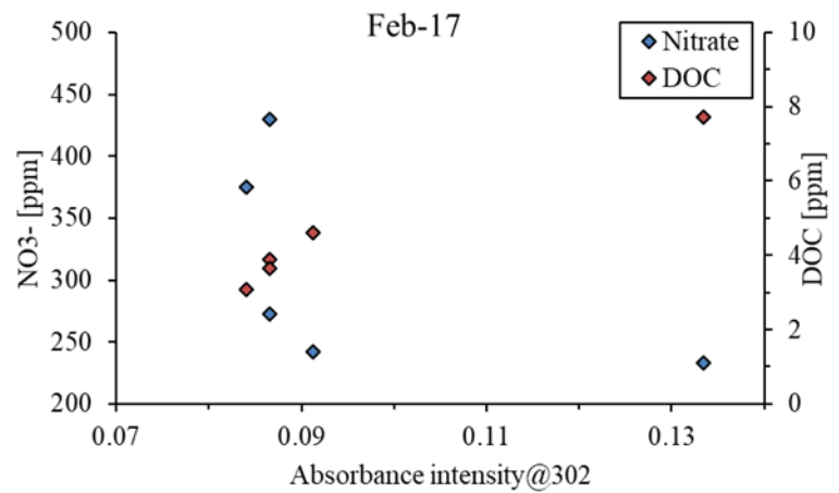
Figure S6 - Anomaly of nitrate spectral analyses at the organic greenhouse samples around 302nm region, during: September – 2015, January and February 2017.
