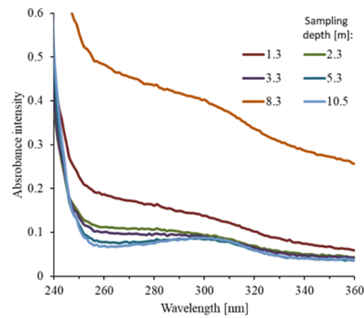
Figure S6 - Anomaly of nitrate spectral analyses at the organic greenhouse samples around 302nm region, during: September – 2015, January and February 2017.
