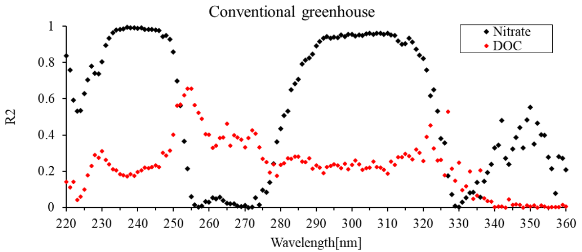
Figure S7 - Organic and conventional greenhouses R^2 vs. wavelength: Note how nitrate concentration in the organic greenhouse can be measured at a narrow range around 230nm, while at the conventional greenhouse nitrate can be measured between 230-240nm and around the 300nm area.
