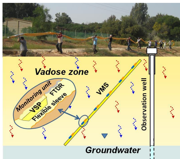
Figure S1 - The Vadose Zone Monitoring System as it is carried prior to its installation (top), and a general layout of the VMS systems when placed in the soil (bottom).
