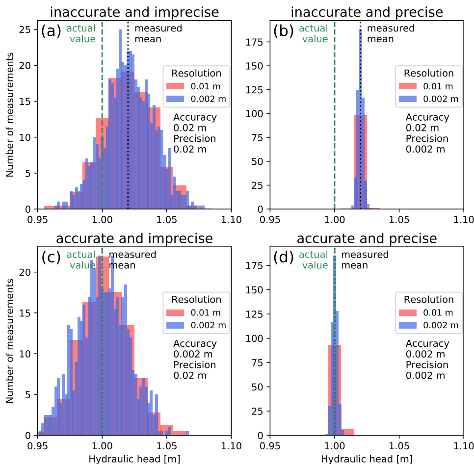
Figure 2. Possible combinations of accuracy, precision and resolution illustrated in a matrix, when 1,000 measurements of the same head ( h = 1 m) are made. Measurements are (a) inaccurate and imprecise, (b) inaccurate and precise, (c) accurate and imprecise, (d) accurate and precise. Examples are illustrated with two different values of accuracy, precision and resolutions (equal to bin width in histogram).
