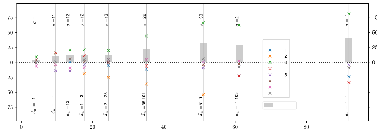
Figure 4. Manual measurement of 9 different groundwater depths using 8 different dip meters: Difference from mean and standard deviation (precision) over mean depth.
