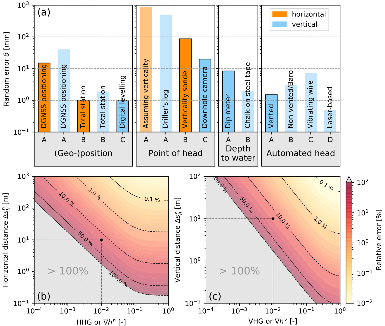
Figure 12. (a) Visual comparison of horizontal and vertical random errors listed as precision values in Table 1 (note that some errors are distance dependent) for the different steps (Figure 1) and method options. Minimum achievable relative random head gradient error in the horizontal (b) and vertical (c) direction calculated using standard practice measurements (highlighted by the black frame: step 1 options A,B,C; step 2 options B,C; step 3 option A; step 4 option A). Note that HHG and VHG values with errors exceeding 100% are blanked out in (b) and (c).
