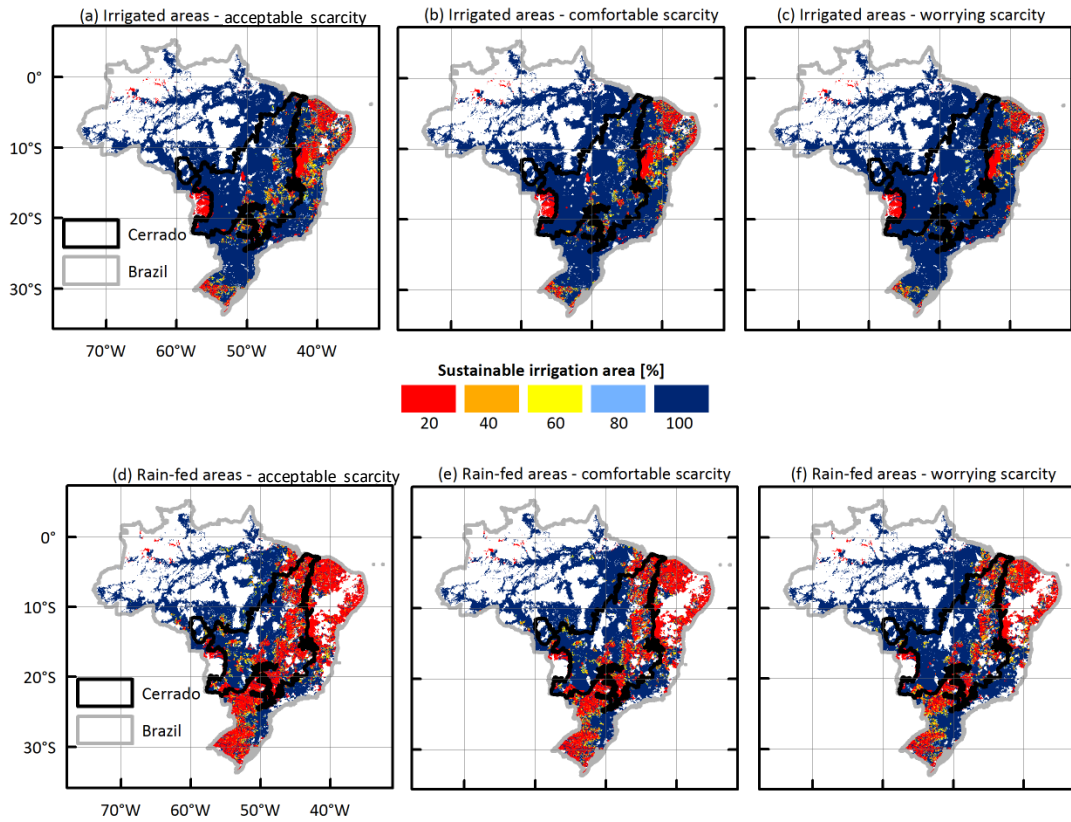
Figure 4. Fraction of current irrigated areas (a,b,c) and potentially irrigated areas (d,e,f) which can be sustainably irrigated according to a target blue water scarcity level of acceptable (a,d), comfortable (b,e) and worrying (c,f).
