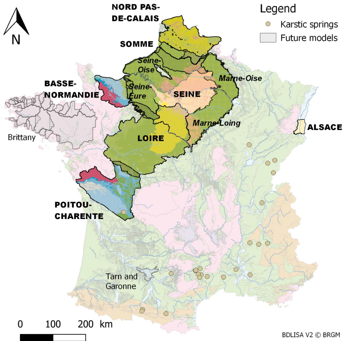
Figure 4: Map of the regional multilayer aquifers and the karstic systems simulated in AquiFR . The outlines of the models are also shown with colours corresponding to the outcropping aquifers with respect to their geological contexts. Grey areas correspond to models that will be integrated in a near future.
