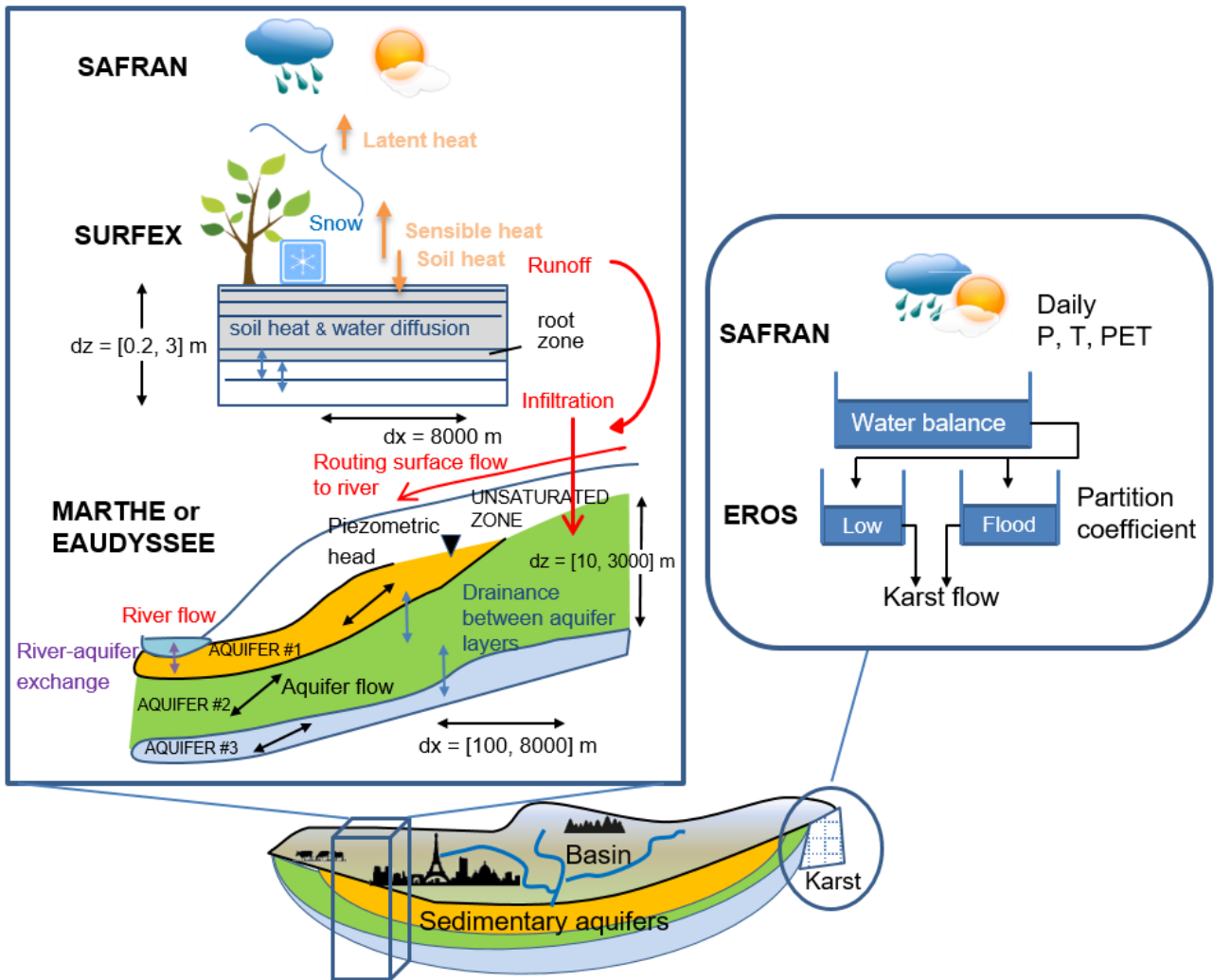
Figure 1: Scheme of the Aquifer physical system. The simulation of the watersheds depends on its hydrogeologic characteristics. For sedimentary basins, the transfer of water within the watersheds is estimated by MARTHE or EauDyssée. It accounts for flows in the unsaturated zones, to (red thin arrow) and in the rivers, in (black arrows) and between (blue arrows) aquifer layers, as well as the exchange between the river and the aquifer (purple arrow). The temporal resolution is daily and the spatial resolution varies from 100 m to a maximum of 8000 m. The depth of the deepest aquifer layer can reach locally about 1000 meters. The 8 km spatial partition of the flow between surface runoff and groundwater recharge (red thick arrows) is estimated by the SURFEX land surface scheme. It solves the water and energy budget at a 5 minutes time step. It accounts for the local type of vegetation and soil, the presence of snow, and a multilayer soil that can reach a depth of 3 meters. The atmospheric forcing is provided by SAFRAN. 5 10 For the karstic systems, the EROS conceptual model is used. It represents each karstic system as lumped basins based on a reservoir approach at a daily time scale. The incoming atmospheric forcing is provided by SAFRAN.
