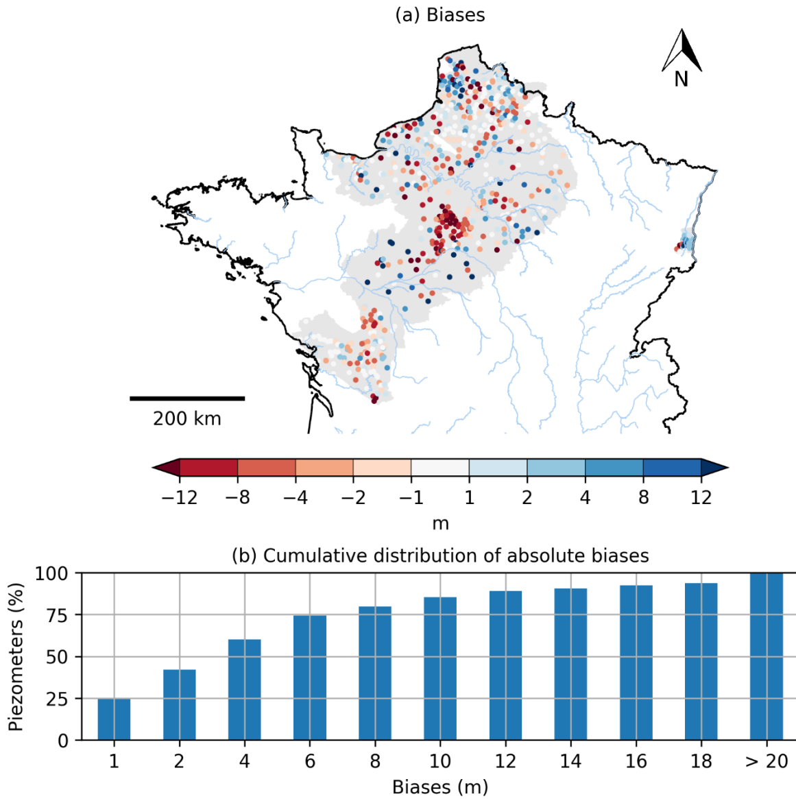
5 Figure 6: (a) Spatial distribution of the biases calculated between the simulated and observed piezometric heads for the 639 selected piezometers. The grey background colour corresponds to the simulated aquifer domain. (b) Cumulative distribution of absolute biases for all the piezometers.
