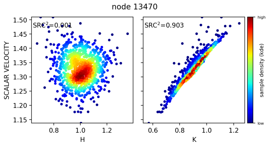
Fig. 3. Scatterplot of scalar velocity for BATT friction formulation.
