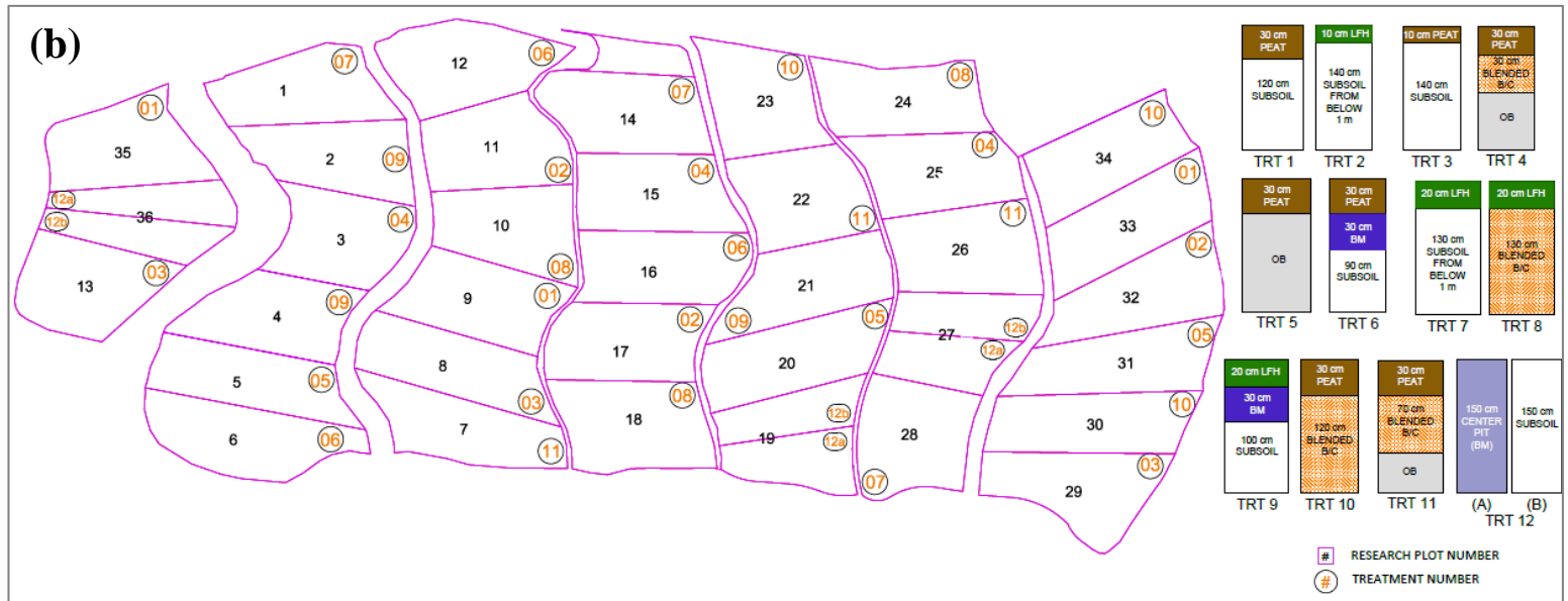
Figure 1: (a) Location map of Aurora North Mine of Syncrude Canada Ltd. and (b) soil cover design treatments (TRT) at ASCS (adapted from OKC, 2017). LOS overburden (OB) underlies all treatments, even though treatments with less than 150 cm total soil cap thickness only show OB
