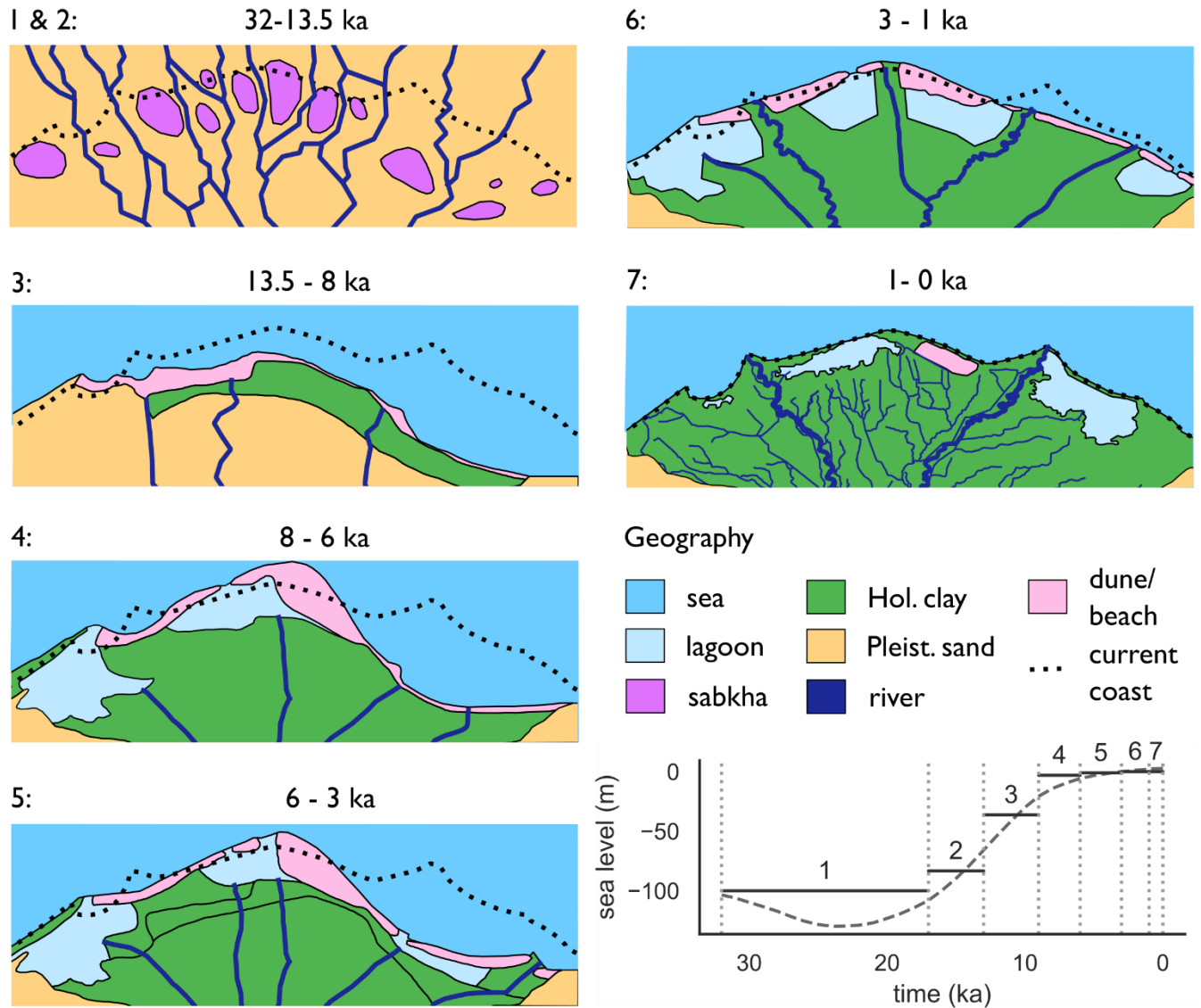
Figure 3: Time slices Stress periods with simplified palaeogeography used as boundary conditions. Figures modified after (Pennington et al., 2017; Stanley and Warne, 1993). The panels focus on the area around the present-day coastline (see Fig. A1 for extent), where upper boundary conditions varied the most. Actual model domain extended beyond the extents of these panels. In the bottom right: The median eustatic sea-level curve (Spratt and Lisiecki, 2016) and the selected sea-level for each time slice stress period .
