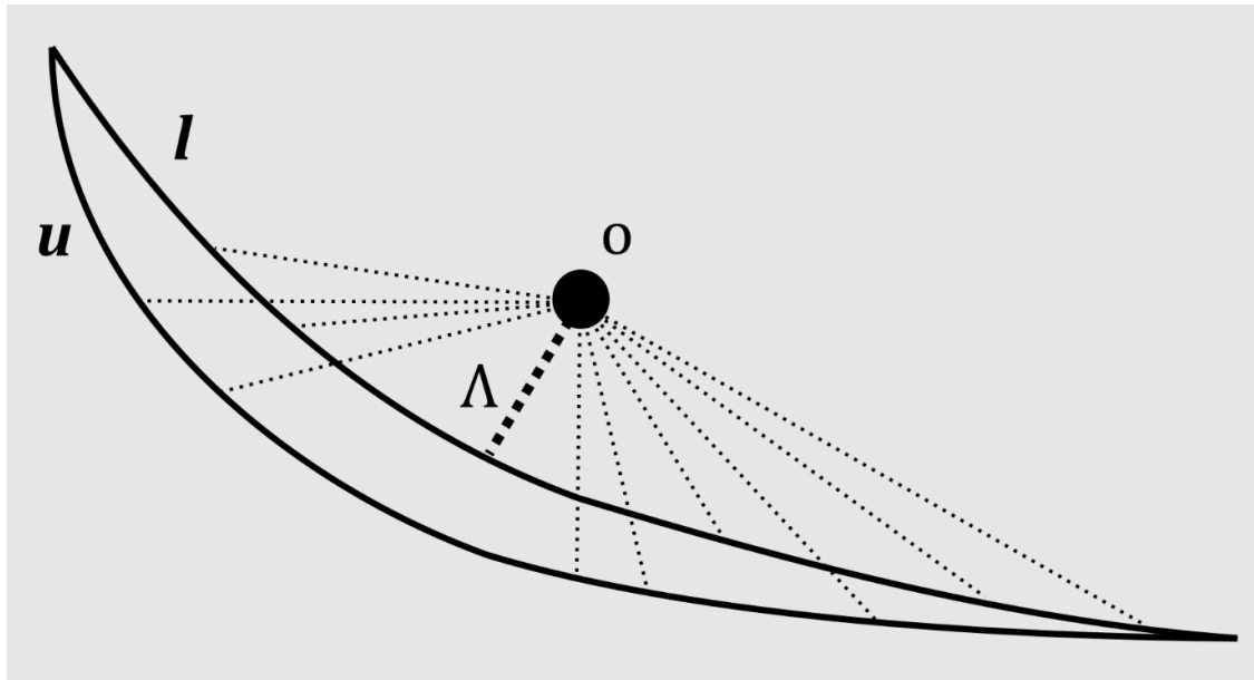
Figure A23: Sketch of how \Lambda is determined with equation 1 for a 2-dimensional example. The circle represents the location of the observation. l and u , the isosurfaces of the lower and upper bound, respectively. The thick dotted line represents the minimum Euclidian distance to an isosurface bound, \Lambda . The thinner dotted lines some other Euclidian distances.
