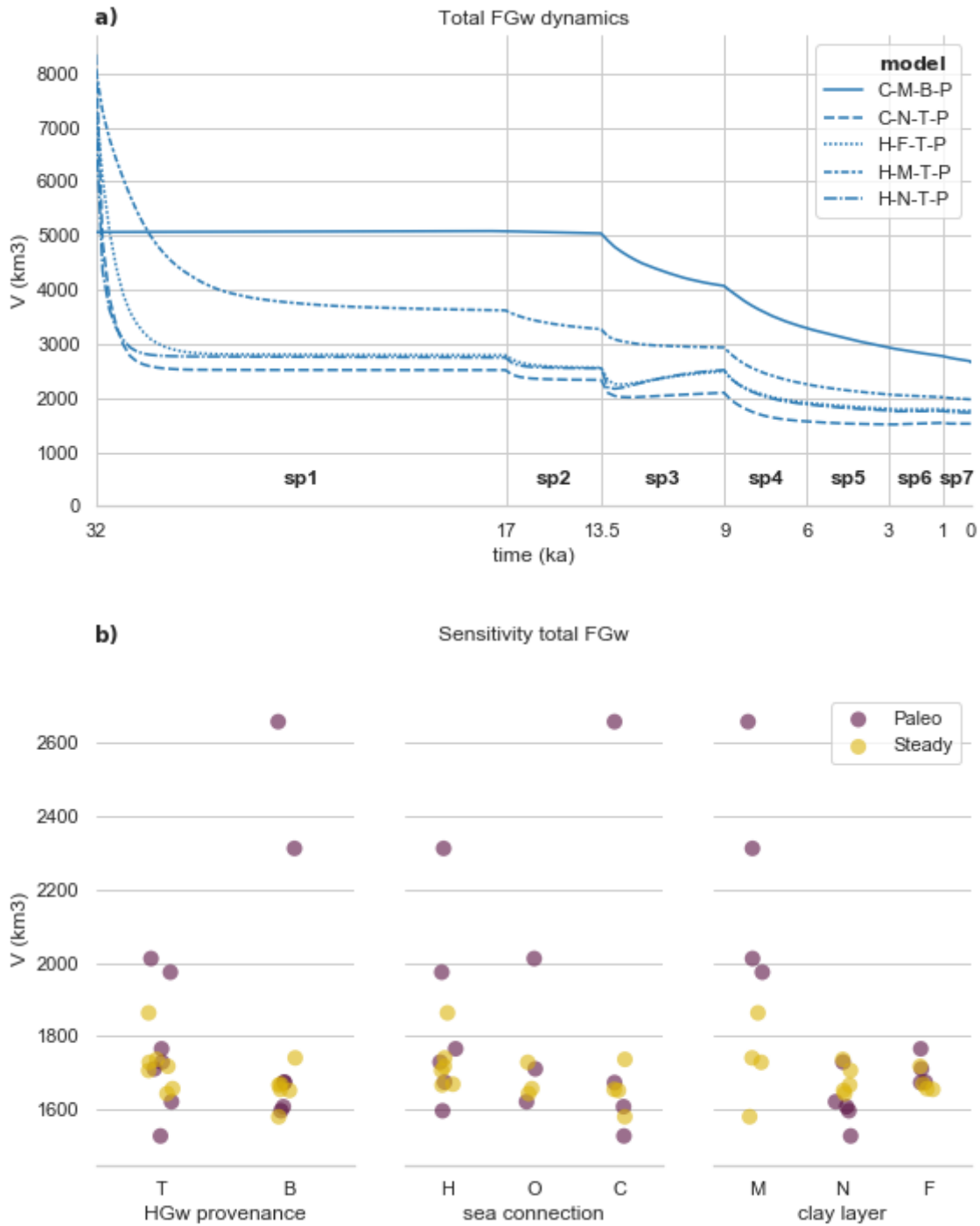
Figure 7: (a) the development of the total FGw volume through time for the five acceptable model scenarios. Time slice Stress period numbers are indicated in bold with “ tssp ”. (b) End state total FGw volumes of all model scenarios, grouped for different inputs. Colours of the dots indicate a steady state or palaeohydrogeological reconstruction result. Dots are jittered to better show overlapping dots.
