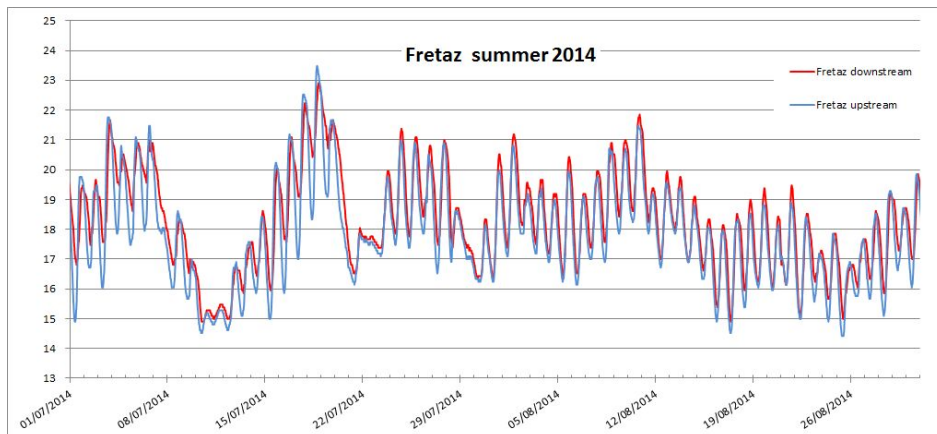
Fig. 3. Figure 2. Time-series of water temperature (°C) upstream (blue) and downstream (red) of the dam Fretaz, Veyle stream, respectively in years 2014 and 2016.
