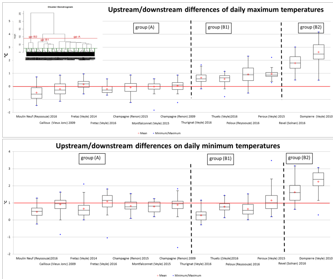
Figure 6. Box-plot distribution (25% - 75 %) of upstream/downstream differences of daily maximum (A) and minimum (B) temperatures for all the time-series studied. (Red lines: 0°C for daily maximum temperature and 1°C for daily minimum temperature are drawn to help reading). The vertical lines drawn in bold are the limits to the three classes of results of the hierarchical cluster analysis. Dendrogram CAH's result is shown at the top left of the figure.
