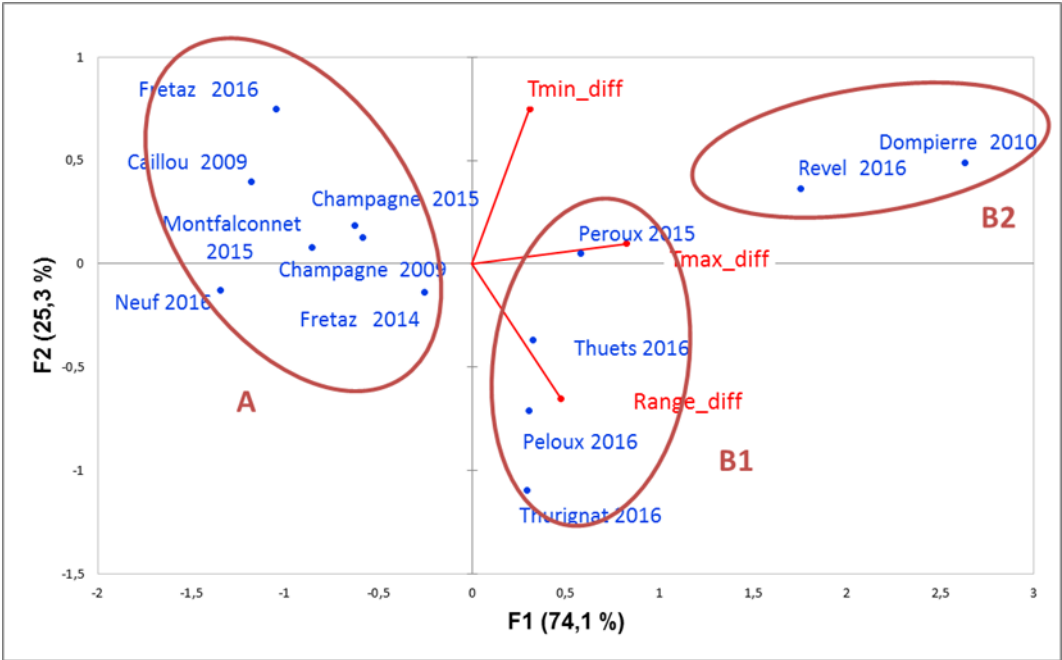
Figure 8. PCA analysis. Scatterplot of time series. Ellipses are drawn to visualize the groups obtained with the hierarchical cluster analysis
