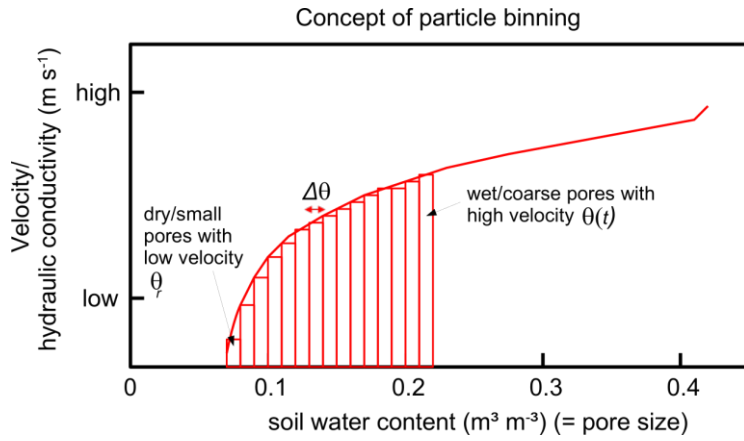
Figure 1. Concept of particle binning. All particles within a grid element are subdivided into bins (= red rectangles) of different pore sizes. Dependent on their related bin the particles travel at different flow velocities.
