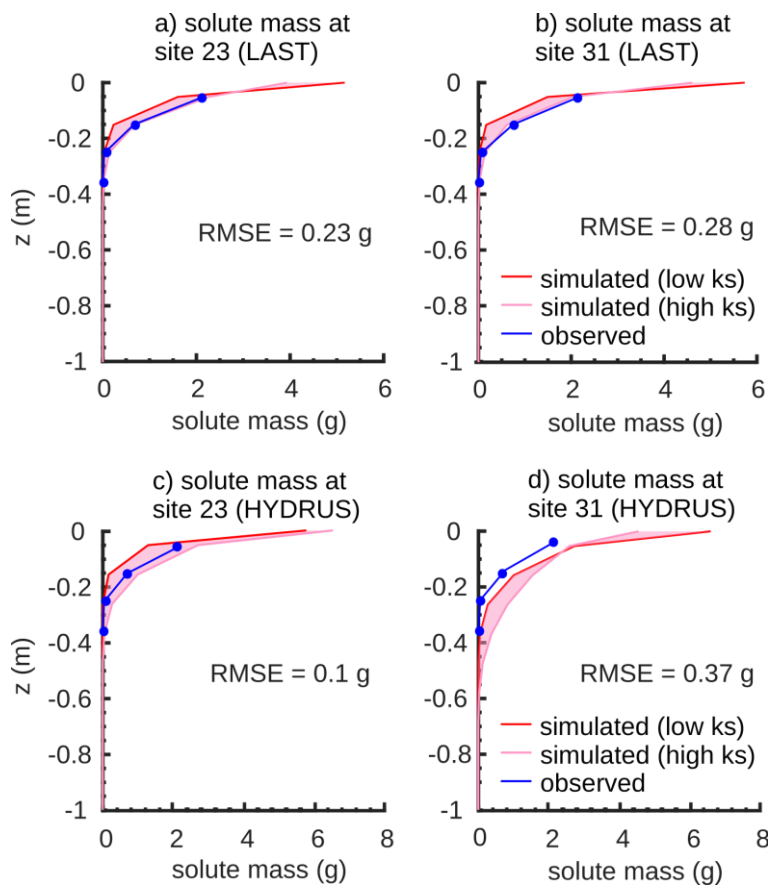
5 Figure 5. Final simulated and observed vertical bromide mass profiles of the matrix at the two well-mixed sites 23 + 31 (a+b) with RMSE values simulated with the LAST-Model. In comparison, final simulated and observed vertical bromide mass profiles at the two well-mixed sites 23+31 (c+d) with RMSE values simulated with HYDRUS 1-D. The rose shaded area shows the uncertainty area of measured k_r values.
