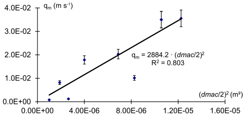
Figure 4. Linear regression of the flux rate within the macropore on the macropore radius ( d_{mac}/2 ) at the study site Spechtacker (edited figure, adopted from Zehe and Flüher, 2001b). This relation was derived from measurements of saturated flow through undisturbed soil columns containing worm burrows.
