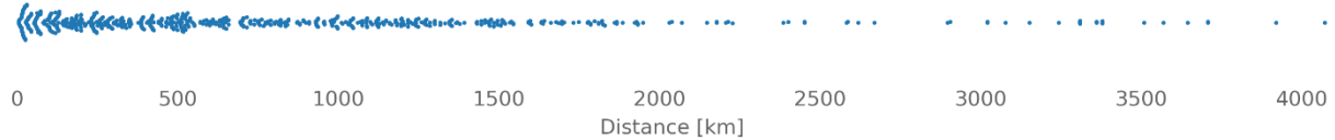
220 Figure 5: Swarm plot of the real world distances of all catchments to the most hydrologically similar catchment (based on their distance in the PCA space of the hydrological signatures).
