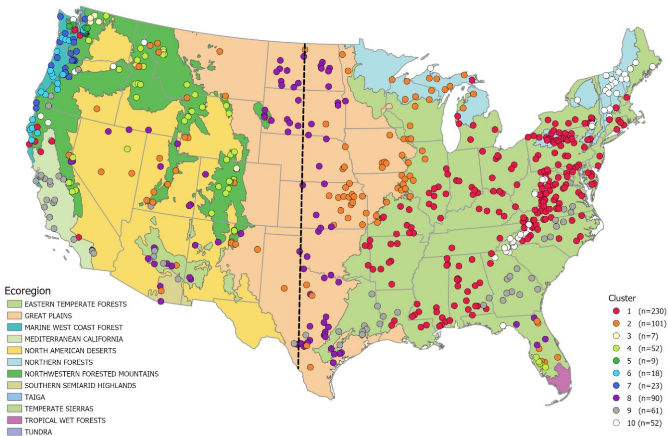
Figure 4: Locations of the clustered CAMELS catchments and level I ecoregions (Omernik and Griffith, 2014) in the continental US. Dotted line marks the 100 th meridian.
