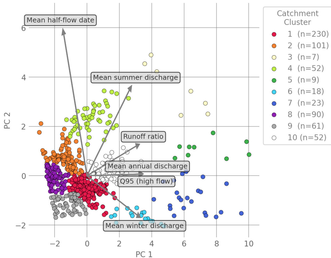
Figure 3: Biplot of the principal components (PC). Colors indicate the cluster of the catchment. Grey arrows indicate the loadings of the original catchment attributes in the PCA space.
