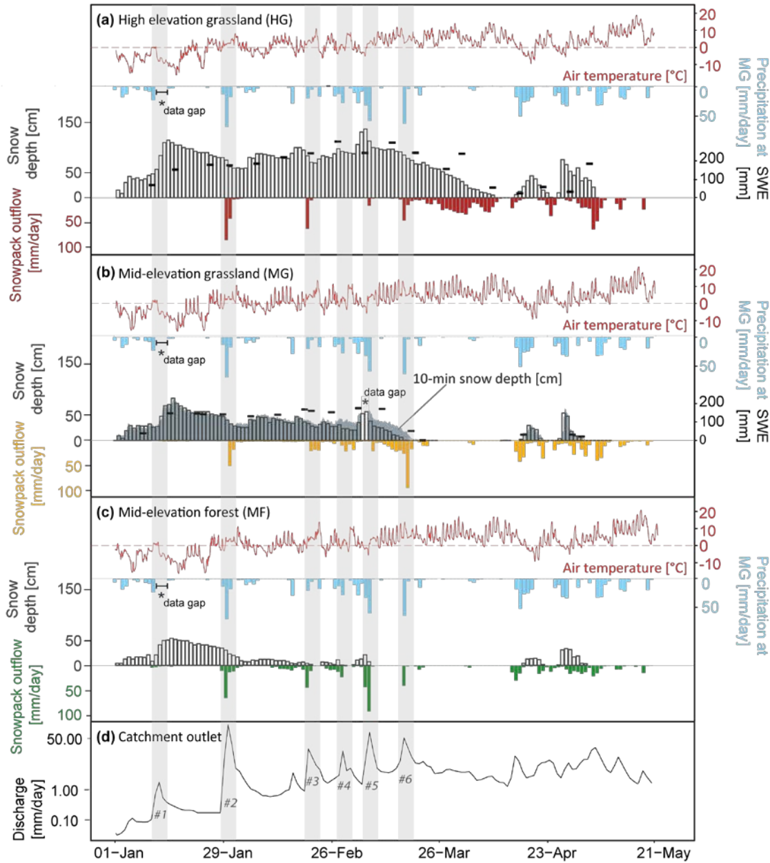
5 Figure 2: Daily precipitation volumes (snow and rainfall) measured at the meteorological station (MG, right axis, panels a-c), along with hourly air temperature, snow depth, snow water equivalent (SWE) and snowpack outflow volumes measured at the high-elevation grassland site (HG, panel a), mid-elevation grassland site (MG, panel b), and mid-elevation forest site (MF, panel c) for the study period 1 January – 22 May 2017. Panel (d) shows daily discharge at the Erlenbach catchment outlet (on log scale). Vertical grey bars indicate the six rain-on-snow (ROS) events that were analysed in this study. Asterisks (*) indicate data gaps. Winter 2018 data are provided in the supplement.
