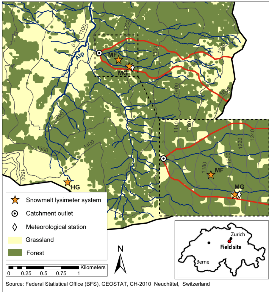
5 Figure 1: The Erlenbach catchment (red outline) in the southern part of the Alptal valley, showing the distribution of vegetation (grassland and forest), as well as the locations of the three snowmelt lysimeter systems (MG: mid-elevation grassland site; MF: mid-elevation forest site; HG: high-elevation grassland site). A meteorological station is located near the MG site. At the Erlenbach catchment outlet, river discharge and precipitation (snow- and rainfall) rates are measured, along with stable water isotopes in stream water and precipitation.
