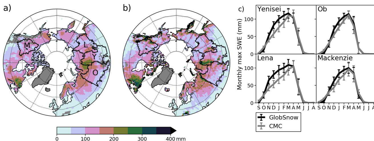
Figure 1. Seasonal maximum SWE (mm) for (a) GlobSnow and (b) CMC for the common overlap period, 2002–2010. The basins used in this study are labelled with their initial (Yenisei, Ob, Lena, Mackenzie). Grey shows regions that are masked. In both data sets Greenland is masked. In addition, GlobSnow pixels are masked where they are more than 50% “mountain”. (c) Mean-monthly climatology averaged over the basins (masked using the GlobSnow mountain mask) for the common overlap period, 2002–2010. Error bars show the inter-annual variability, defined as the standard deviation between years.
