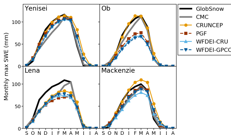
Figure 6. Climatology of monthly maximum SWE (mm) from observations and from the GRC model runs for the common overlap period, 2002–2010.
