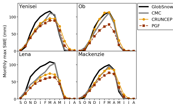
Figure 7. Climatology of monthly maximum SWE (mm) from observations and from the UCC model runs for the common overlap period, 2002–2010.
