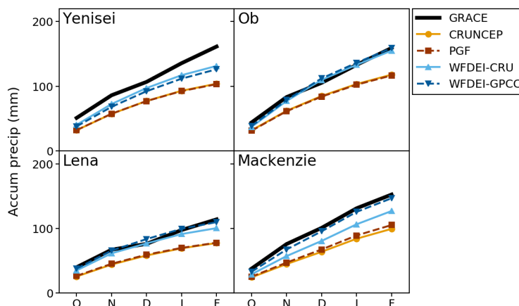
Figure 2. Mean monthly accumulated cold season precipitation in October–February inclusive, averaged over the common overlap period, 2002–2010, as derived from GRACE TWS (Sect. 4) and from the driving data sets (Sect. 2.1).
