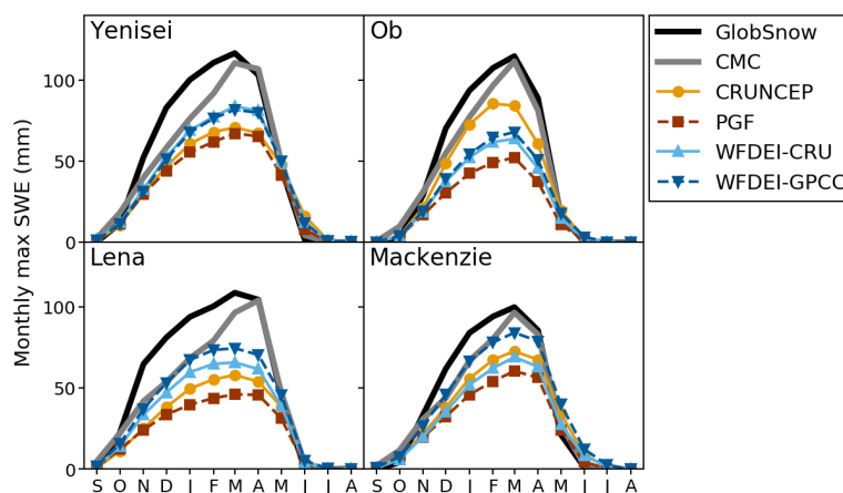
Figure 3. Climatology of monthly maximum SWE (mm) from observations and from the CTL model runs averaged over the common overlap period, 2002–2010.
