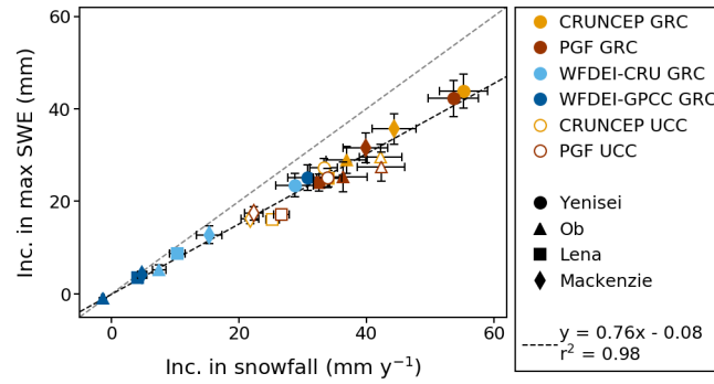
Figure 8. Increase in annual maximum SWE (mm) from CTL to GRC and UCC runs compared to increase in annual snowfall ( \text{mm y}^{-1} ), averaged over all basins (using the GlobSnow mountain mask for snowfall as well as SWE) for each driving data set. This is averaged over the whole of each JULES run (see Table 1).
