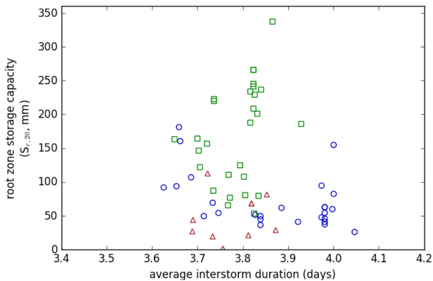
Fig. 1. Average interstorm duration in relation to derived root zone storage capacities, different symbols indicate different boreal regions (green = south boreal; blue = mid boreal; red = north boreal)
