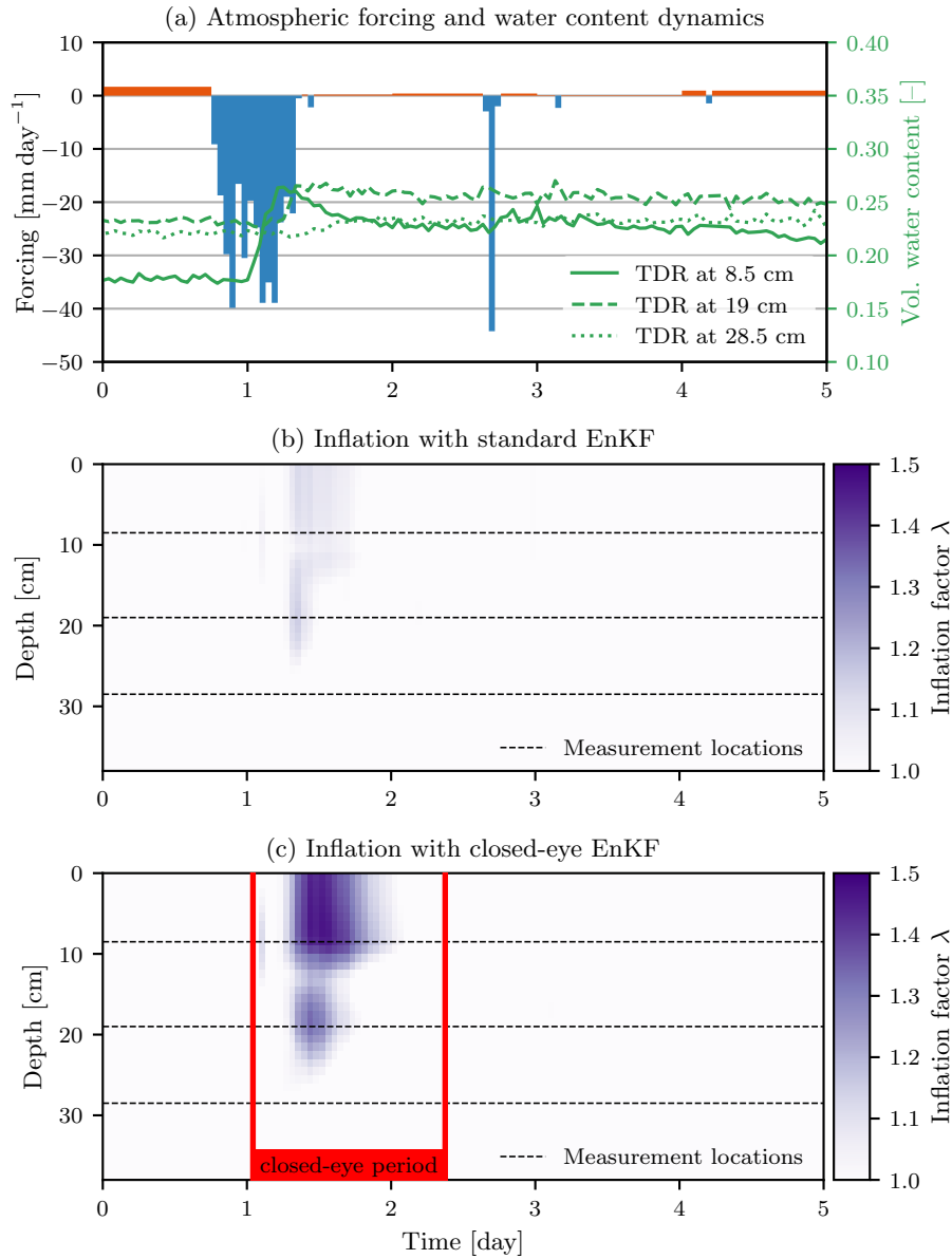
Figure B1. Inflation factor for the water content state in a real-world application for a standard and closed-eye EnKF together with atmospheric forcing and corresponding response of measured water contents. The closed-eye period starts when the infiltration front reaches the topmost TDR. During this time the local equilibrium assumption of the Richards equation is violated and a strong inflation is required. The new inflation method allows a fast adjustment of the inflation factors, which enables the EnKF to effectively guide the water content states with the TDR measurements through the closed-eye period. Modified from Bauser (2018).
