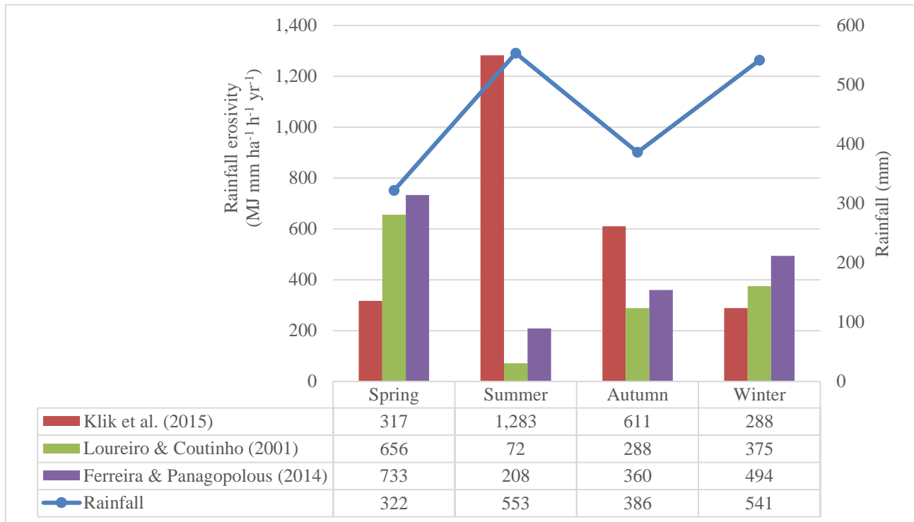
15 Figure 1: Graph of seasonal rainfall and estimates of erosivity in the Mangatarere.
