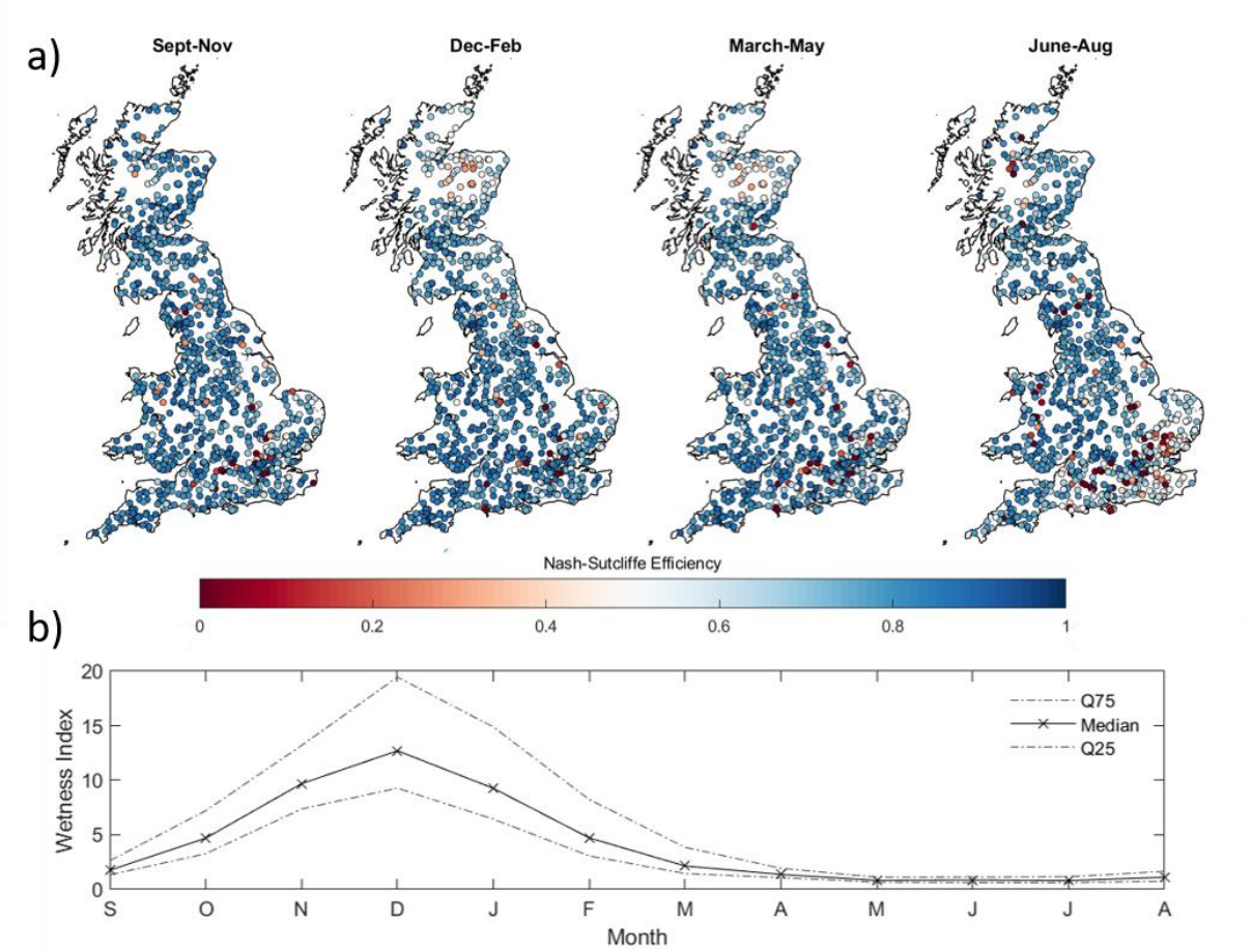
Figure 7: GB maps of FUSE multi-model ensemble model performance for each season (4a) and observed seasonal variations in catchment wetness index (4b). Each point on 4a is a gauge location which is coloured based upon the best Nash Sutcliffe score attained by any of the four models sampled for that catchment and season. Figure 4b then shows how seasons vary hydrologically across GB, through the wetness index (precipitation/PET) calculated from the observed data, split by month, used to drive the hydrological models across all catchments shown in 4a.
