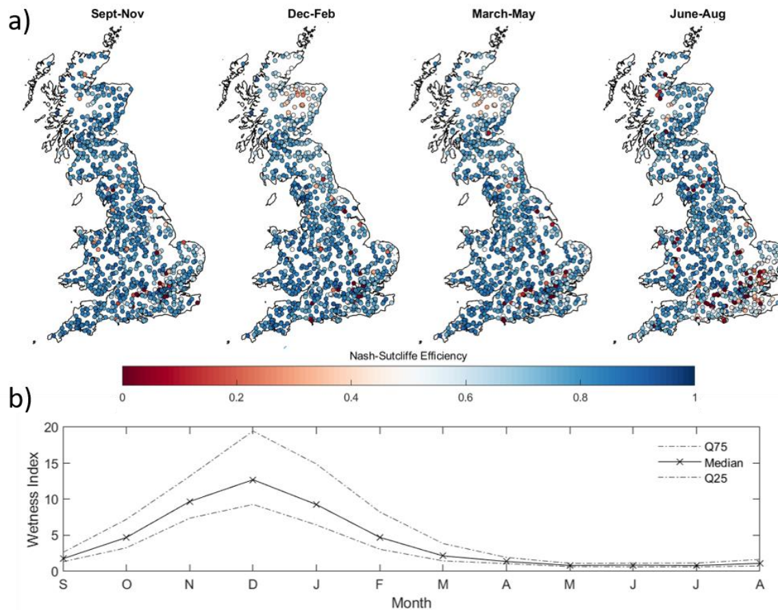
Figure 6: GB maps of FUSE multi-model ensemble model performance for each season (4a) and observed seasonal variations in catchment wetness index (4b). Each point on 4a is a gauge location which is coloured based upon the best Nash Sutcliffe score attained by any of the four models sampled for that catchment and season. Figure 4b then shows how seasons vary hydrologically across GB, through the wetness index (precipitation/PET) calculated from the observed data, split by month, used to drive the hydrological models across all catchments shown in 4a.
