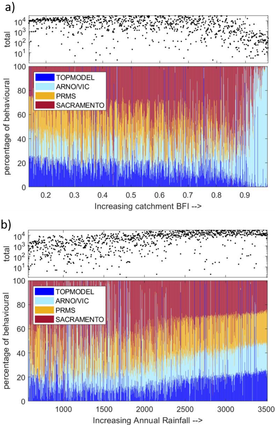
Figure 7: Relative performance of the four FUSE model structures, depending on catchment characteristics. Scatter plots show the total number of behavioural simulations, from all model structures, forming each line on the stacked bar graph. Each line on this stacked bar chart represents 1 catchment, and the colour shows the proportion of the behavioural simulations from each model structure. Catchments have been ordered by BFI (a) and Annual Rainfall (b).
