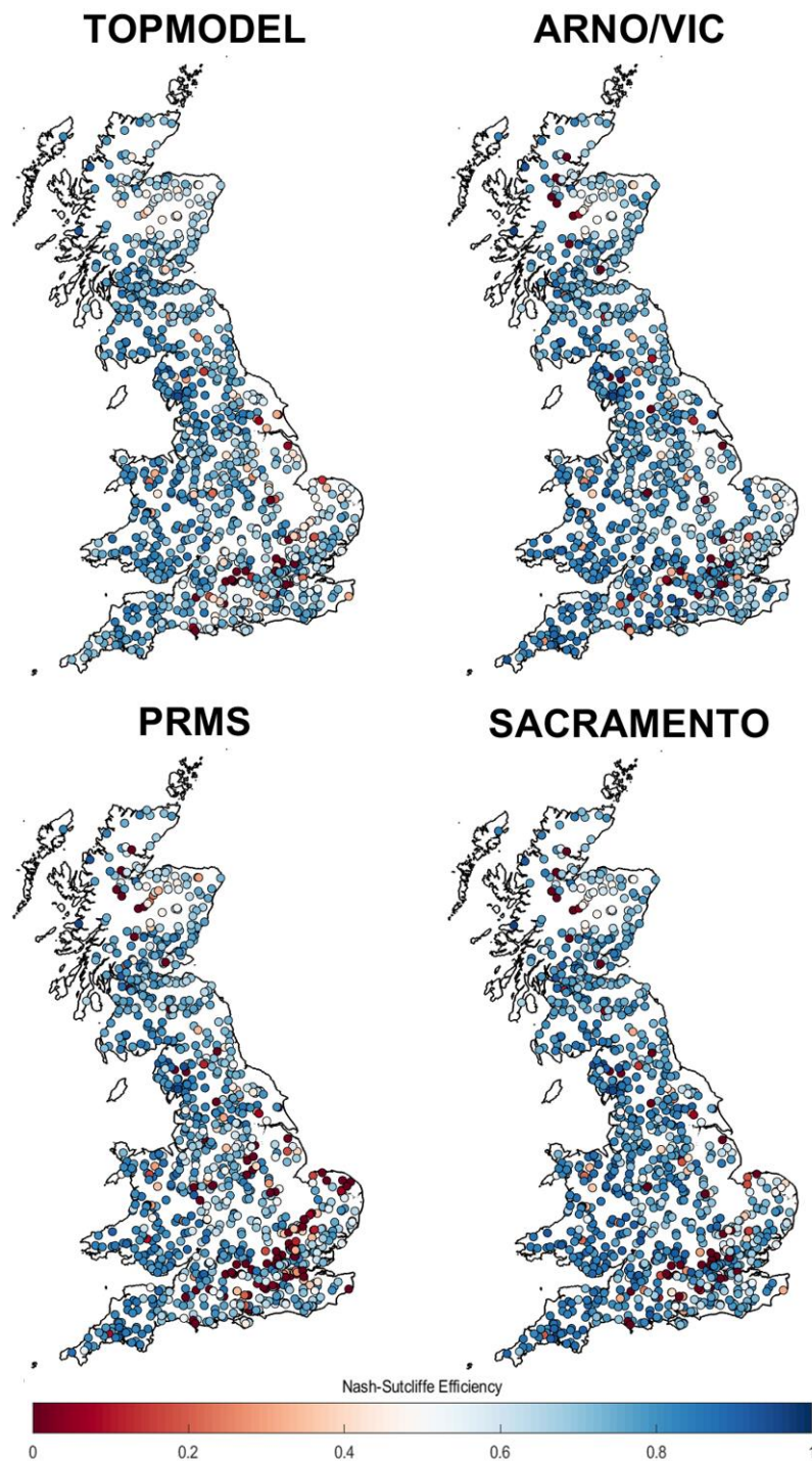
Figure 4: GB maps of model performance for each structure. Each point is a gauge location which is coloured based upon the best Nash Sutcliffe score attained by the model for that catchment.
