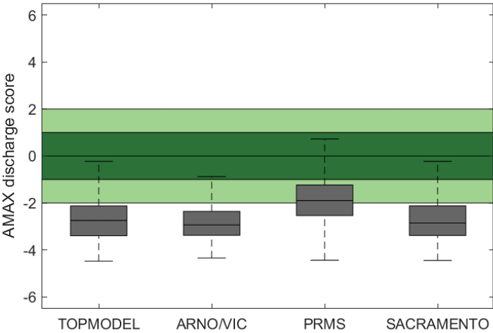
Figure 10: Predictive capability of 4 hydrological models for annual maximum (AMAX) flows across Great Britain. Shows behavioural model ensemble (NSE>0.5) median performance in replicating the observed AMAX flows, with a value of 0 being a perfect score and a value of 1 meaning the simulated AMAX value was at the limits of the observational uncertainty. The spread covers all catchments.
