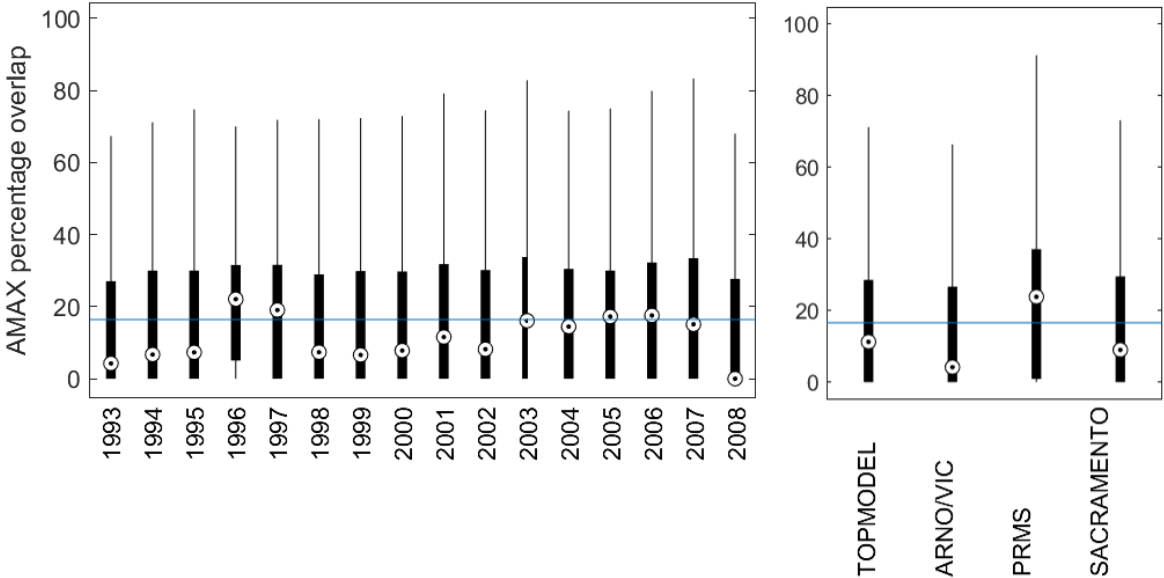
Figure 11: Predictive capability of 4 hydrological models for annual maximum (AMAX) flows across Great Britain. Boxplots show the overlap of the simulated and observed uncertainty bounds, as a percentage of the total uncertainty. This metric ranges from 0 to 100, with 0 indicating no overlap between observed and simulated AMAX discharge and 100 indicating a perfect overlap of observed and simulated discharge bounds. The range in the left plot is over all catchments and all models, whilst the right-hand plot shows the range across all catchments.
