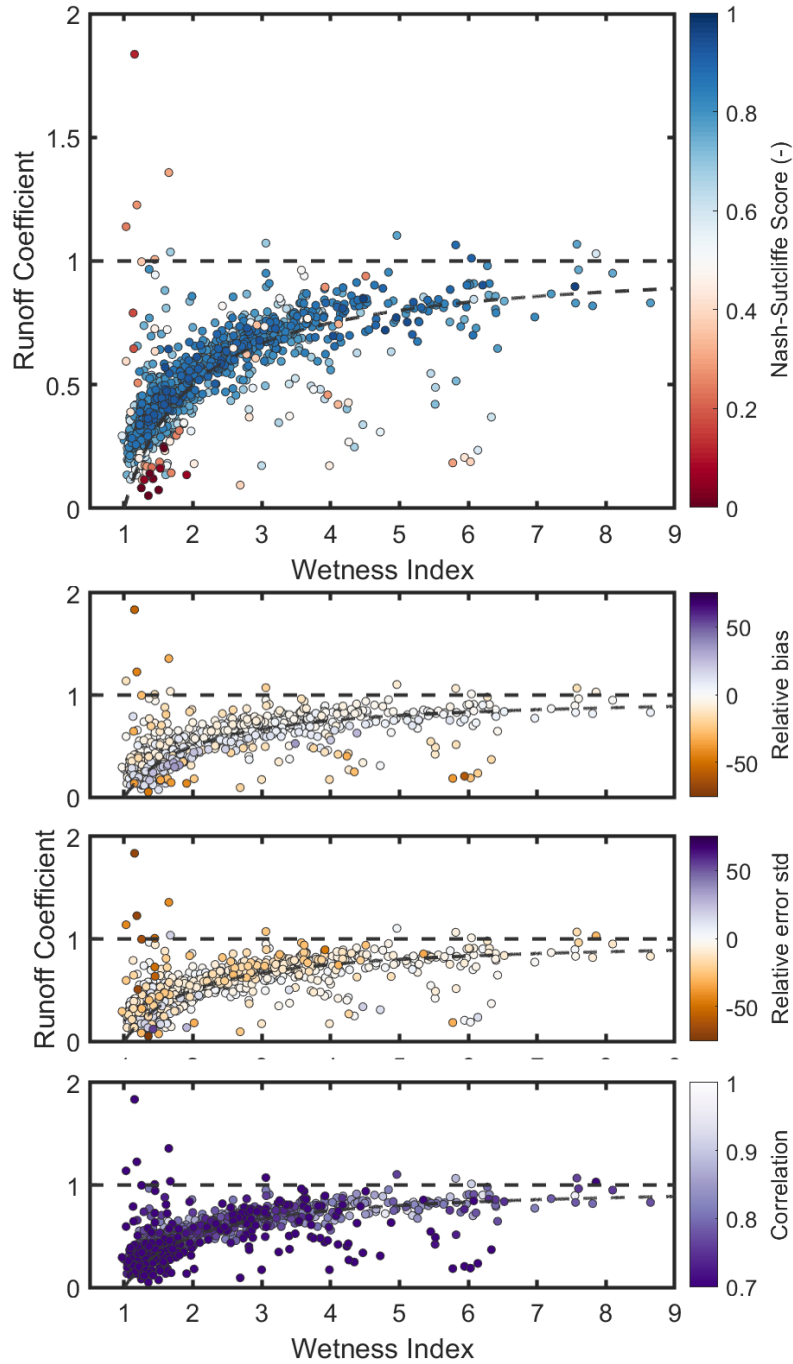
Figure 9: Scatter plots of the relationship between wetness index, runoff coefficient and best sampled model performance. Each point represents a catchment, coloured by the best Nash-Sutcliffe score for that catchment from the model structure ensemble. The plotting order was modified to ensure catchments with more extreme (high and low) performance values would be plotted on top. Any points above the horizontal dotted line are where runoff exceeds total rainfall in a catchment and any points below the curved
