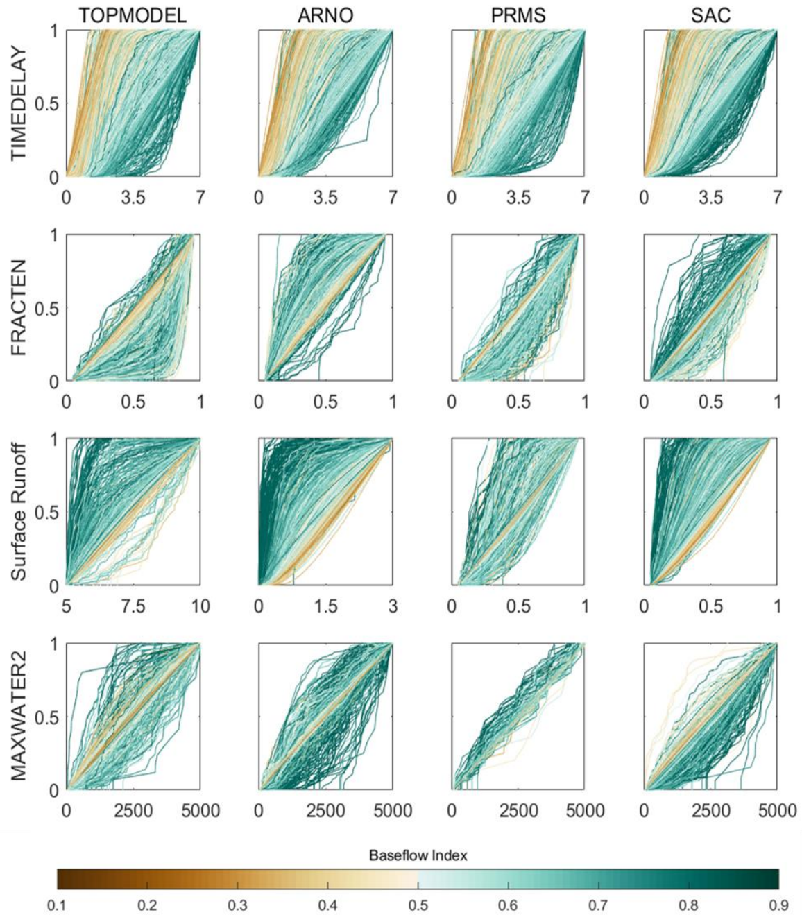
Figure 8: Cumulative distribution function (CDF) plots showing parameter values of the behavioural simulations for each catchment. Each line represents a catchment and is coloured by that catchment's BFI. The 4 rows show different parameters controlling different parts of the hydrograph. Surface runoff is given by the LOGLAMB (TOPMODEL), AXV_BEXP (ARNO) and SAREMAX (PRMS and SAC) as there was no common surface runoff parameter used for all 4 models. Each column is a different hydrological model.
