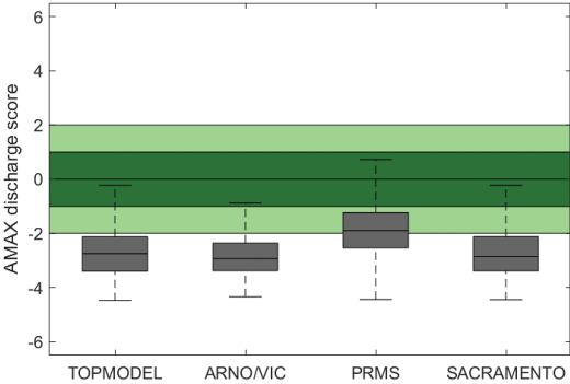
Figure 1140: Predictive capability of 4 hydrological models for annual maximum (AMAX) flows across Great Britain. Shows behavioural model ensemble ( NSE > 0.5 ) median performance in replicating the observed AMAX flows, with a value of 0 being a perfect score and a value of 1 meaning the simulated AMAX value was at the limits of the observational uncertainty. The spread covers all catchments.
