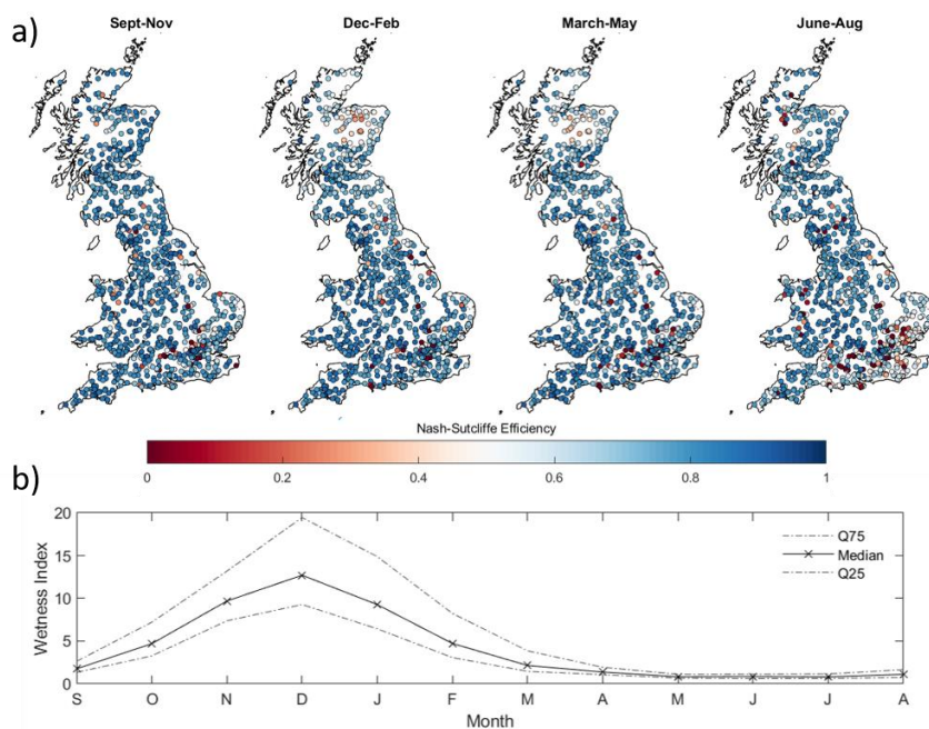
Figure 7: GB maps of FUSE multi-model ensemble model performance for each season (47a) and observed seasonal variations in catchment wetness index (74b). Each point on 4a is a gauge location which is coloured based upon the best Nash Sutcliffe score attained by any of the four models sampled for that catchment and season. Figure 47b then shows how seasons vary hydrologically across GB, through the wetness index (precipitation/PET) calculated from the observed data, split by month, used to drive the hydrological models across all catchments shown in 74a.
