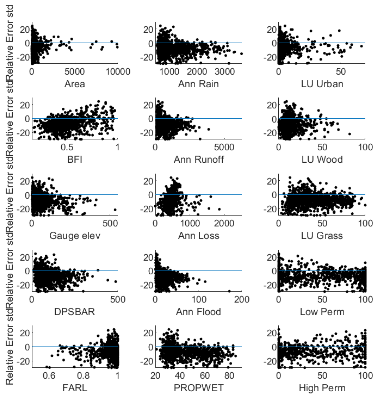
Figure S3: Relationship between error in standard deviation and a selection of 15 catchment descriptor variables, as in Figure S1.
