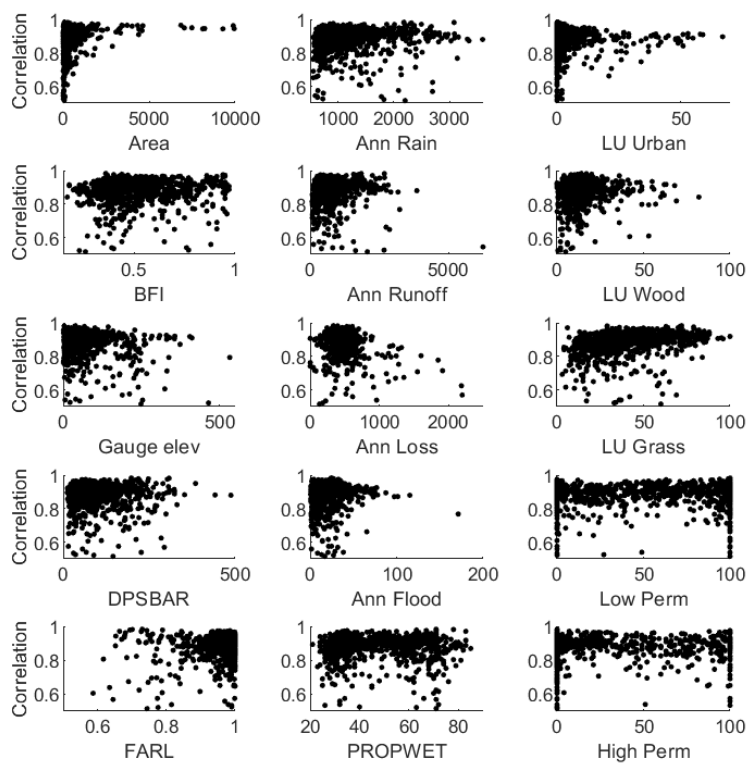
Figure S4: Relationship between correlation and a selection of 15 catchment descriptor variables, as in Figure S1.
