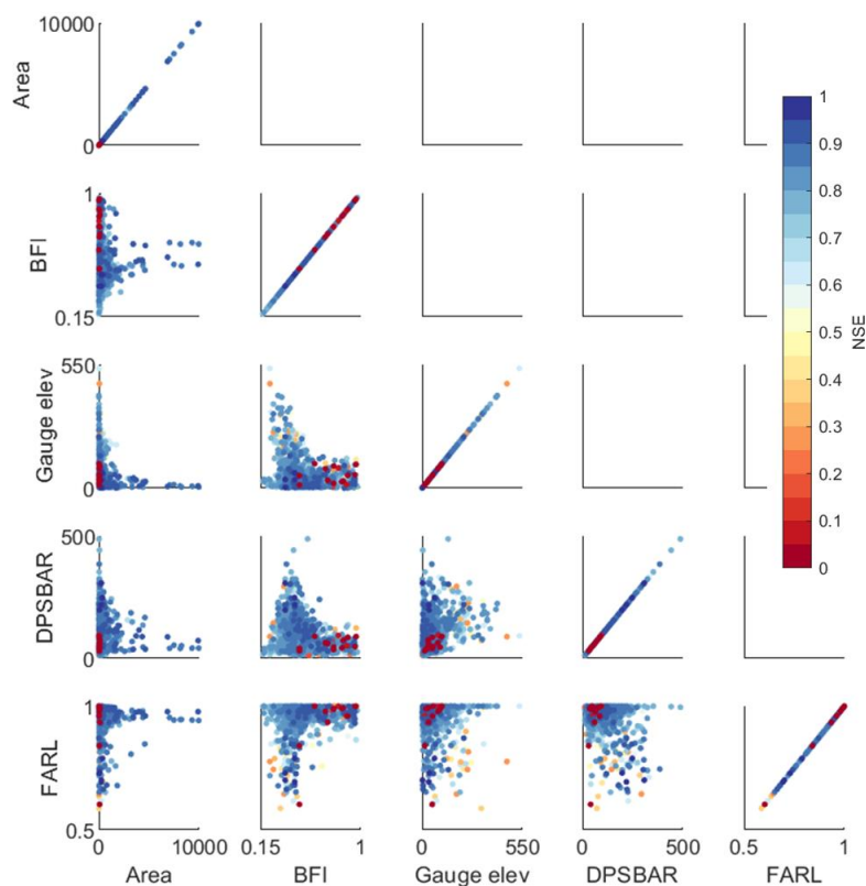
Figure S5: Relationship between general catchment characteristics, coloured by model ensemble NSE score for that catchment. Column 1 gives general catchment attributes from the hydrometric register (Marsh and Hannaford, 2008). These are catchment area (km 2 ), Baseflow index (BFI), Gauge elevation (m above sea level), mean drainage path slope (DPSBAR) which indicates overall catchment steepness in metres per kilometre, and flood attenuation by reservoirs and lakes (FEARL) where values close to 1 indicate the absence of flow attenuation and values below 0.8 indicate a substantial influence. Column 2 gives hydroclimatic attributes calculated from our data, and proportion catchment is wet (PROPWET) from the hydrometric register. Annual Loss is Rainfall-Runoff, whilst Annual flood is the Median Annual maximum flood peak, and all are reported in mm. Column 3 gives land-use and bedrock permeability descriptors (%), also from the UK hydrometric register.
