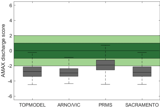
Figure 11: Predictive capability of 4 hydrological models for annual maximum (AMAX) flows across Great Britain. Shows behavioural model ensemble ( NSE > 0.5 ) median performance in replicating the observed AMAX flows, with a value of 0 being a perfect score and a value of 1 meaning the simulated AMAX value was at the limits of the observational uncertainty. The spread covers all catchments.
