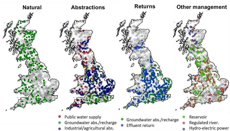
Figure 1. Factors affecting runoff in the study catchments, using information from the UK hydrometric register. Natural catchments are defined as having limited variation from abstractions/discharges so that the gauged flow is within 10% of the natural flow at or above the Q_{95} flow. The groundwater category includes both groundwater abstraction and recharge, as well as the few catchments where mine-water discharges influence flow. Full descriptions of all factors can be found in the UK hydrometric register (Marsh and Hannaford, 2008b).
