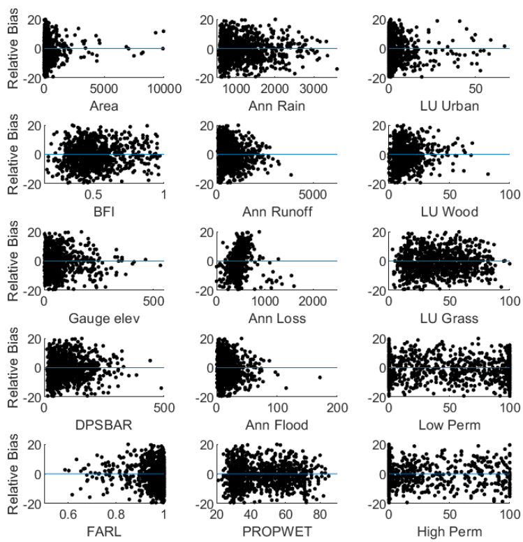
Figure S2: Relationship between bias and a selection of 15 catchment descriptor variables, as in Figure S1.
