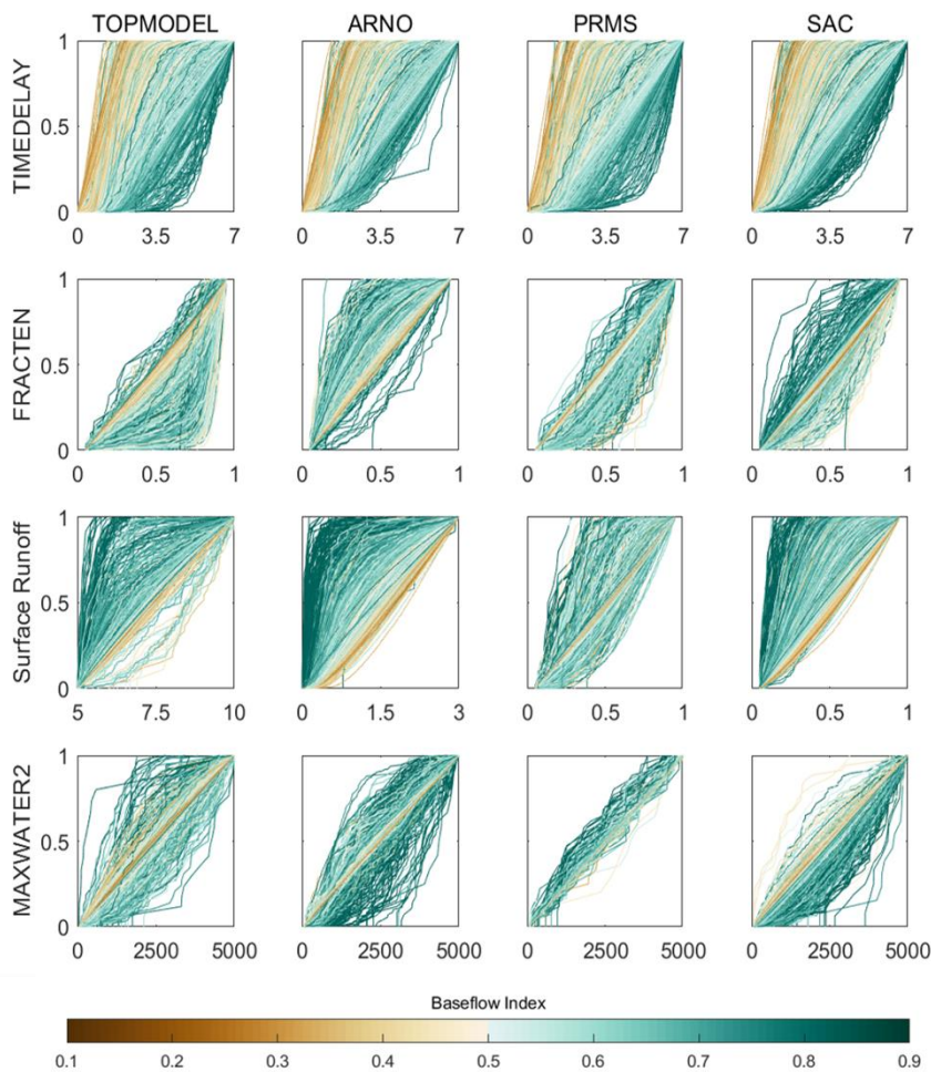
Figure 98: Cumulative distribution function (CDF) plots showing parameter values of the behavioural simulations for each catchment. Each line represents a catchment and is coloured by that catchment's BFI. The 4 rows show different parameters controlling different parts of the hydrograph. Surface runoff is given by the LOGLAMB (TOPMODEL), AXV_BEXP (ARNO) and SAREMAX (PRMS and SAC) as there was no common surface runoff parameter used for all 4 models. Each column is a different hydrological model.
