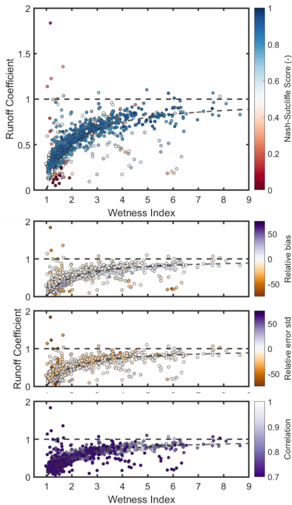
Figure 109: Scatter plots of the relationship between wetness index, runoff coefficient and best sampled model performance. Each point represents a catchment, coloured by the best Nash-Sutcliffe score for that catchment from the model structure ensemble. The plotting order was modified to ensure catchments with more extreme (high and low) performance values would be plotted on top.
