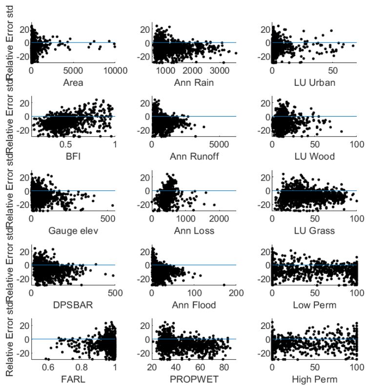
Figure S4S3: Relationship between error in standard deviation and a selection of 15 catchment descriptor variables, as in Figure S2S1.
