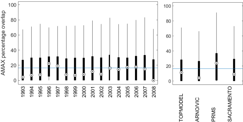
Figure 1244: Predictive capability of 4 hydrological models for annual maximum (AMAX) flows across Great Britain. Boxplots show the overlap of the simulated and observed uncertainty bounds, as a percentage of the total uncertainty. This metric ranges from 0 to 100, with 0 indicating no overlap between observed and simulated AMAX discharge and 100 indicating a perfect overlap of observed and simulated discharge bounds. The range in the left plot is over all catchments and all models, whilst the right-hand plot shows the range across all catchments.
