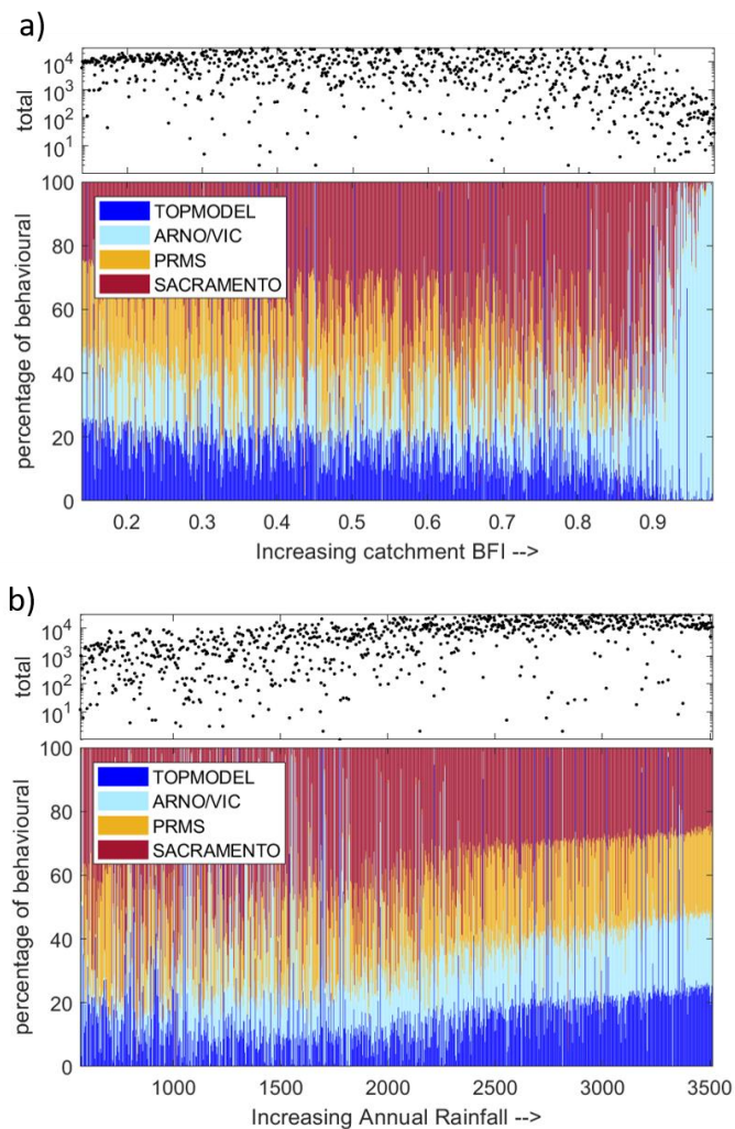
Figure 87: Relative performance of the four FUSE model structures, depending on catchment characteristics. Scatter plots show the total number of behavioural simulations, from all model structures, forming each line on the stacked bar graph. Each line on this stacked bar chart represents 1 catchment, and the colour shows the proportion of the behavioural simulations from each model structure. Catchments have been ordered by BFI (a) and Annual Rainfall (b).
