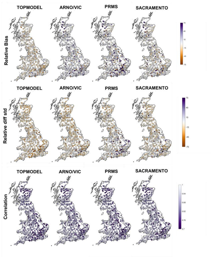
Figure 65. GB maps of model performance for each structure for 3 different metrics. Top row shows model relative bias or relative error in simulated mean runoff (%), middle row shows relative error in the standard deviation of runoff (%), and the third row shows correlation between observed and simulated streamflow. Each point is a gauge location which is coloured based upon the best score for that metric.
