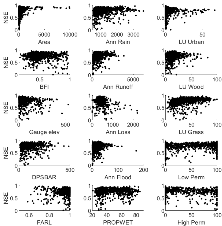
Figure S12: Relationship between NSE and a selection of 15 catchment descriptor variables. Column 1 is more gives general catchment attributes from the hydrometric register (Marsh and Hannaford, 2008). These are catchment area (km 2 ), Baseflow index (BFI), Gauge elevation (m above sea level), mean drainage path slope (DPSBAR) which indicates overall catchment steepness in metres per kilometre, and flood attenuation by reservoirs and lakes (FARL) where values close to 1 indicate the absence of flow attenuation and values below 0.8 indicate a substantial influence. Column 2 gives hydroclimatic attributes calculated from our data, and proportion catchment is wet ( PROPWET ) from the hydrometric register. Annual Loss is Rainfall-
