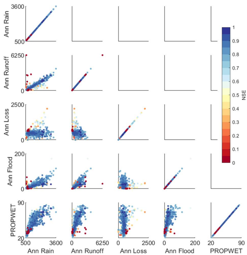
Figure 7aS6. Same as figure S6S5, but this time looking at hydroclimatic catchment descriptors. Annual rainfall (mm), annual runoff (mm), annual loss (mm) and mean annual maximum flood (mm), were all calculated from the model input data used in
