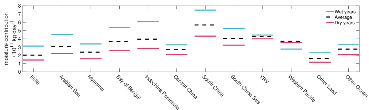
Figure 10. Moisture contribution during the five driest (1981, 1985, 2003, 2013) and wettest (1993, 1995, 1996, 1998, 1999) summers. The average contribution for all summers is also shown with dashed lines. The extent of the source regions are defined in Fig. 4.
