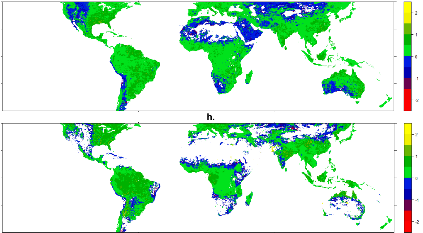
65 Fig. 7: Values of \log_{10}(\epsilon_{x_j}) , where \epsilon_{x_j} is the total uncertainty in variable X (eqn 3), where X is 66 evapotranspiration (a, c, e, f) or runoff (b, d, g, h) and j refers to either high extremes (a, b, e, g) or low 67 extremes (c, d, f, h). Points on the scatter plots are coloured according to latitudinal zones (Fig. 1). Because 68 of the density of overlapping points, only the envelope of points for each latitudinal zone is shown and the 69 points with the highest uncertainty (uncertainty DIU \geq (2/3) * (\text{global maximum of } DIU) ). Linear regression 70 lines for each latitudinal zone indicate the trend as precipitation increases within each zone (all regressions 71 were significant at the 1% level), although n.b. we do not contend in any way that the distribution of points 72 shown is linear: these lines simply indicate a trend that is not clear to the eye from the envelopes displayed 73 (which do not show the complete point cloud). Maps (e-h) show the corresponding spatial distributions of 74 \log_{10}(\epsilon_{x_j}) values for each variable, with the colour scales corresponding to the vertical axis on scatter plot (a). 75
