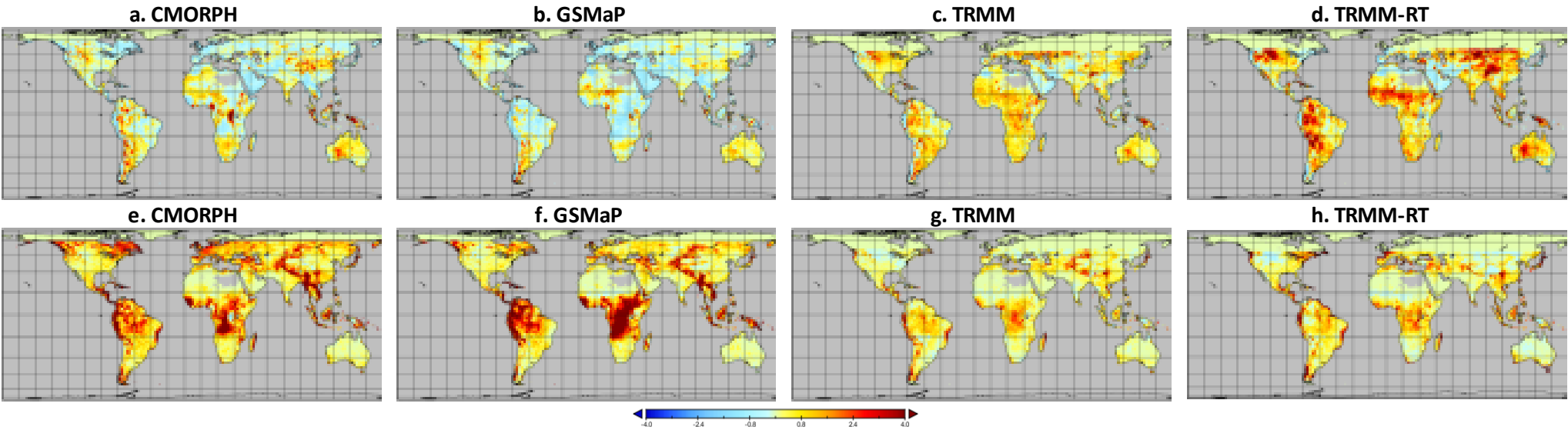
Fig. 4: Increase in extreme precipitation event occurrence in relation to MSWEP. Subtracting extreme high event occurrence rates in the MSWEP precipitation input from the rates in the CMORPH precipitation input gives map (a), and (b) to (d) are the same calculation using GSMaP, TRMM and TRMM-RT instead of CMORPH. (e) to (h) is the same calculation, but for extreme low event occurrence (i.e. the averages of the upper and lower rows are effectively the maps Fig. 3a and Fig. 3b, respectively). The clear lines at 50°N (TRMM, TRMM-RT) and 60°N (CMORPH, GSMaP) show the bounds of data validity for these products (Table 2). Note that only isolated global areas exceeded 4 events/yr, so the scale is restricted to -4 to +4 events/yr.
