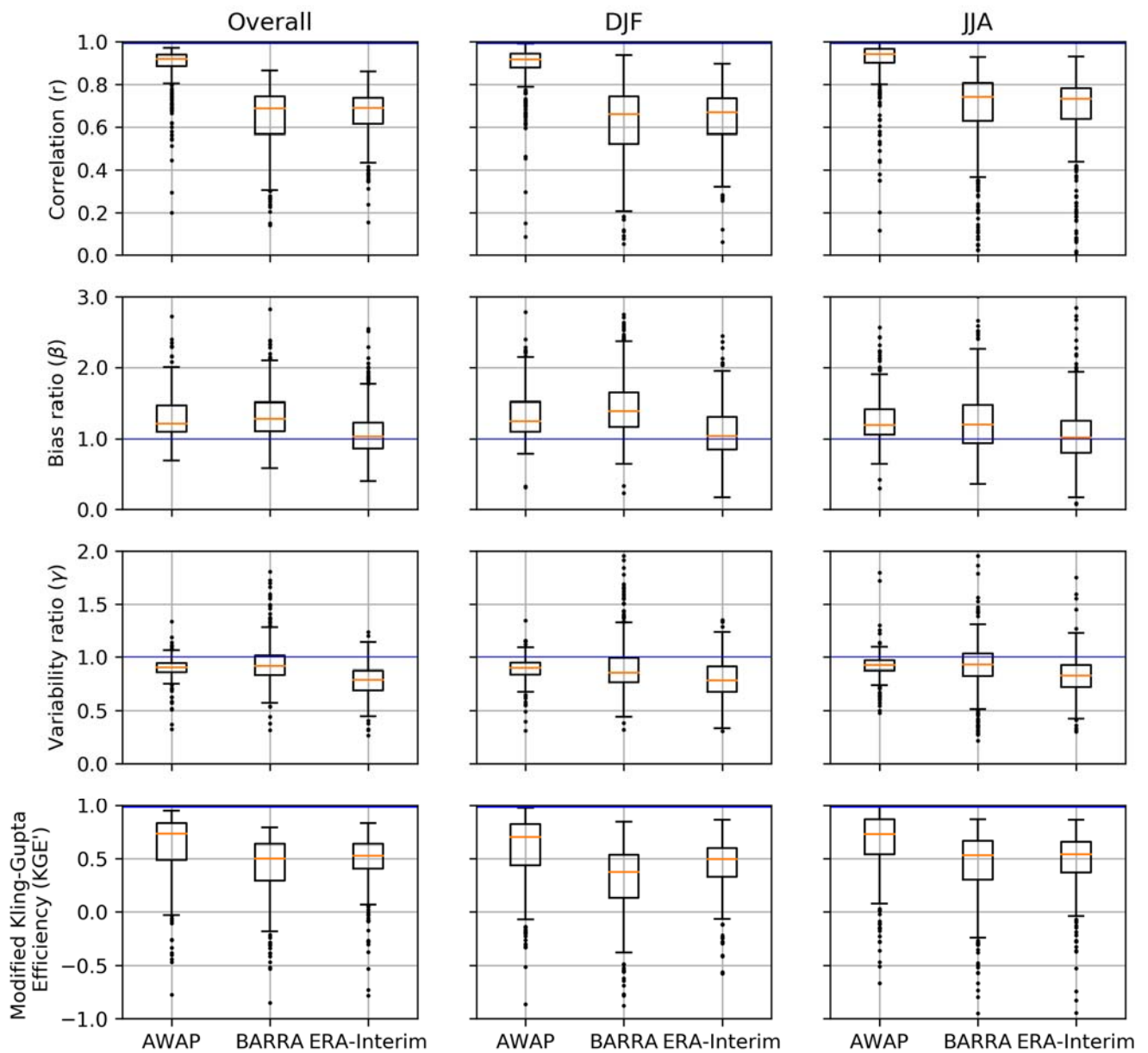
5 Figure 3 Boxplot of correlation ( r ), bias ratio ( \beta ), variability ratio ( \gamma ), and modified Kling-Gupta Efficiency (KGE') between daily precipitation estimates from gridded datasets and observations at gauge locations. Columns represent overall data, summer (DJF), and winter (JJA) respectively. Each box extends from first to third quartile, medians are marked in each box, and whisker extends to furthest point or 1.5 times the interquartile range whichever is closer. The blue horizontal line represents the best value.
