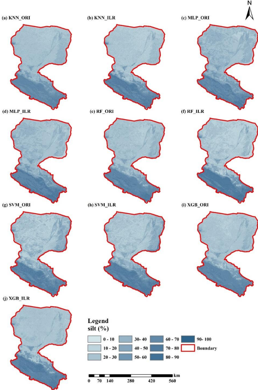
Figure S1. The interpolation maps of silt fraction.
