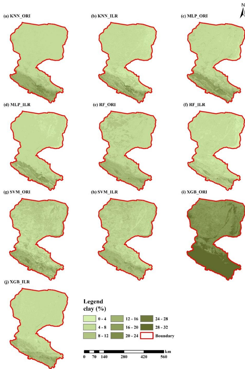
Figure S2. The interpolation maps of clay fraction.
