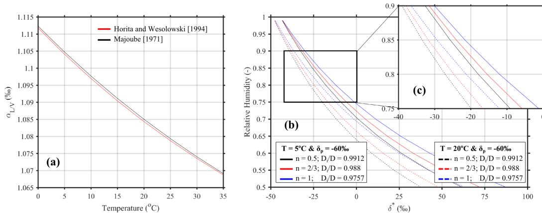
Fig. 1. a) Estimation of \alpha_{L/V} (fractionation parameter) against temperature, b) The estimation of \delta^* , c) subplot of plot b
