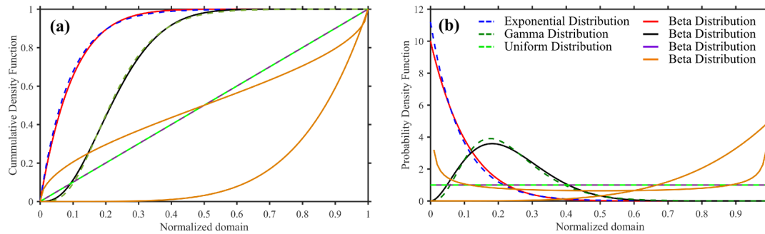
Fig. 2. a) The CDF of an exponential, gamma, and uniform distribution with a corresponding beta distribution parameterisation. b) The corresponding PDF of the CDFs in Fig2.a
