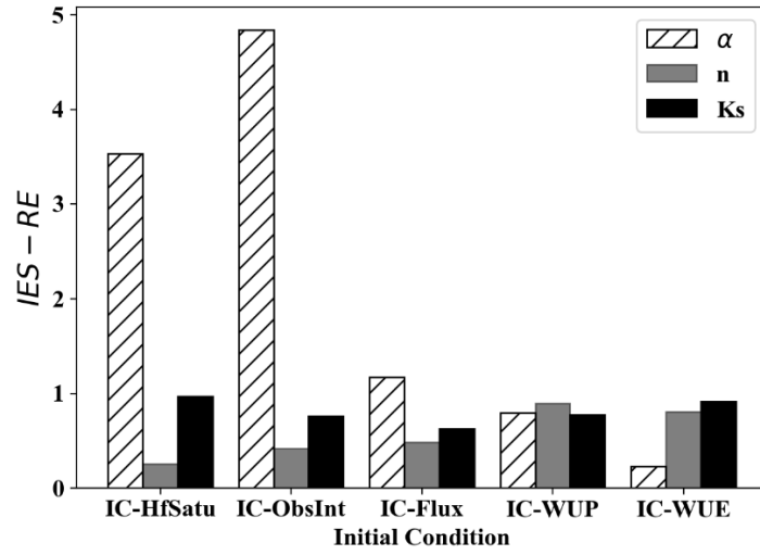
Fig. 9. The RE results of parameter estimations under five initialization methods with IES when the simulation time is 60 days (Case 5).
