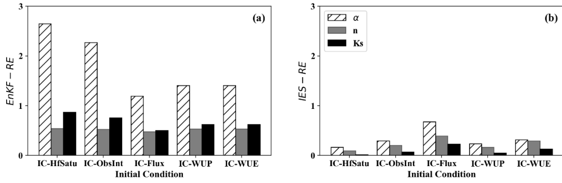
815 Fig. 8. The RE results of parameter estimations ( \alpha , n and K_s ) under five initialization methods with (a) EnKF and (b) IES (Case 4).
