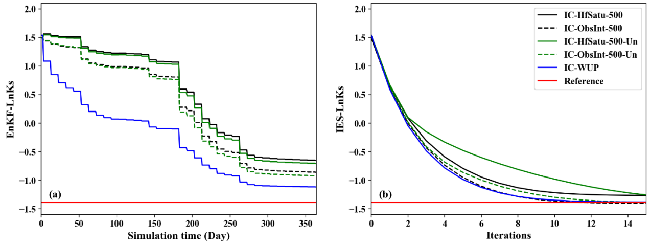
Fig. 7. The impacts of increased ensemble size (Case 2) and uncertainty of initial state (Case 3) on the results of \ln K_s estimations within EnKF and IES.
