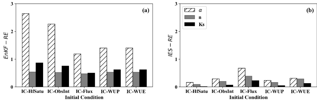
Fig. 8. The RE results of parameter estimations ( \alpha , n and K_s ) under five initialization methods with (a) EnKF and (b) IES (Case 4).
