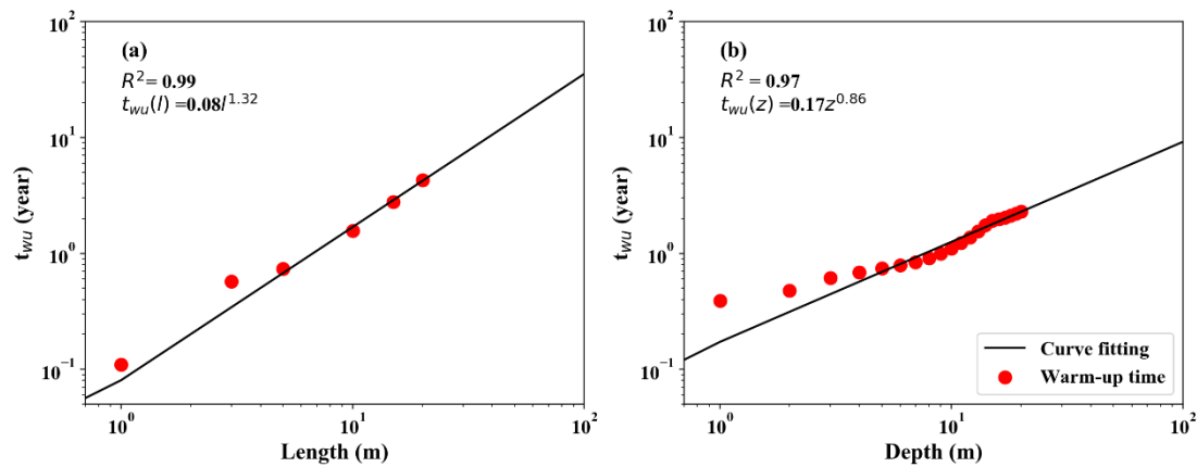
Fig. 5. (revised manuscript) The value of the warm-up time t_{wu} . (a) The overall profile t_{wu} values versus different soil profile lengths ( l ) and (b) t_{wu} value as a function of depth z with a 20-m soil profile.
