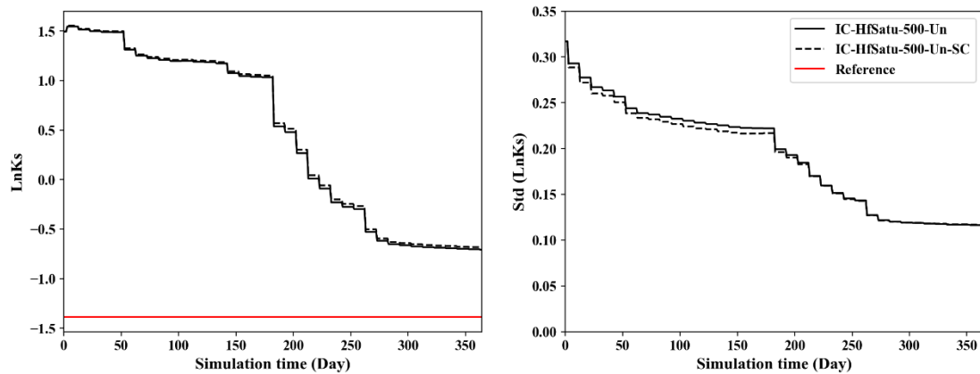
Figure 1. The results of \ln K_s estimation and their associated standard deviations with IC-HfSatu-500-Un and IC-HfSatu-500-Un-SC.
