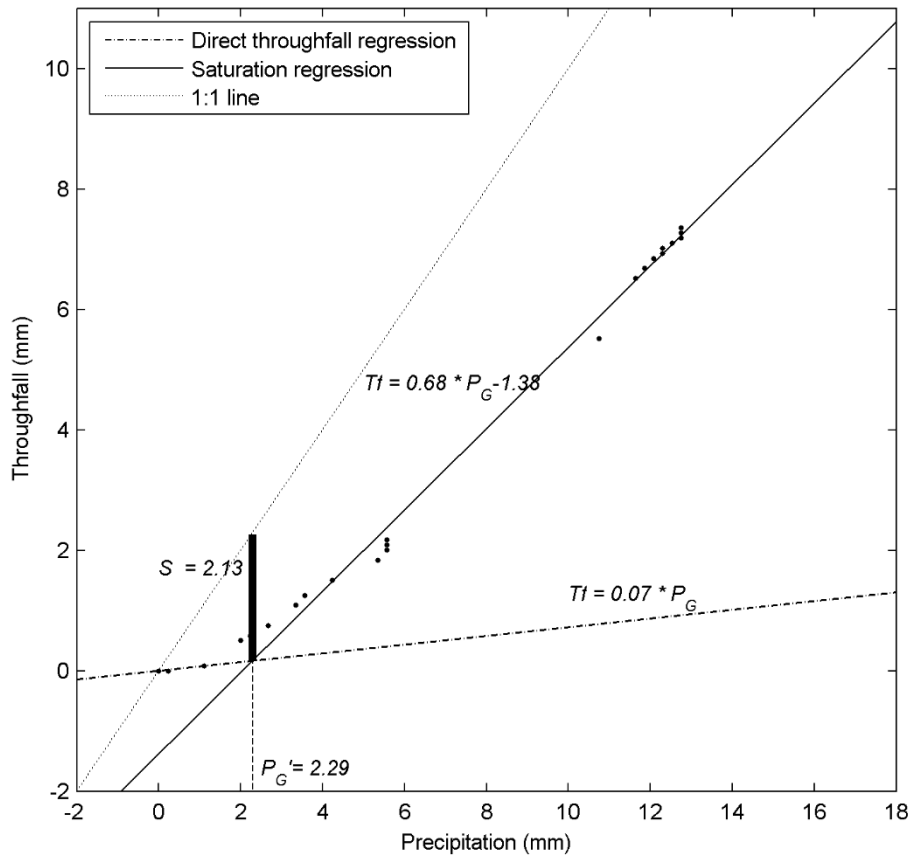
Figure 5. Example of individual event analysis (IEA) on 17 September 2015, plot of data used to estimate canopy direct throughfall and saturation storage capacity, assuming no evaporation during the wetting phase. Dots represent values of cumulative rainfall versus cumulative Tf . The direct throughfall regression equation for this particular event was Tf = 0.07 P_G . The saturation regression equation was Tf = 0.68 P_G - 1.38 . Canopy saturation point ( P'_G ) was calculated as the intersection of the two linear regressions, P'_G = 2.19 mm.
