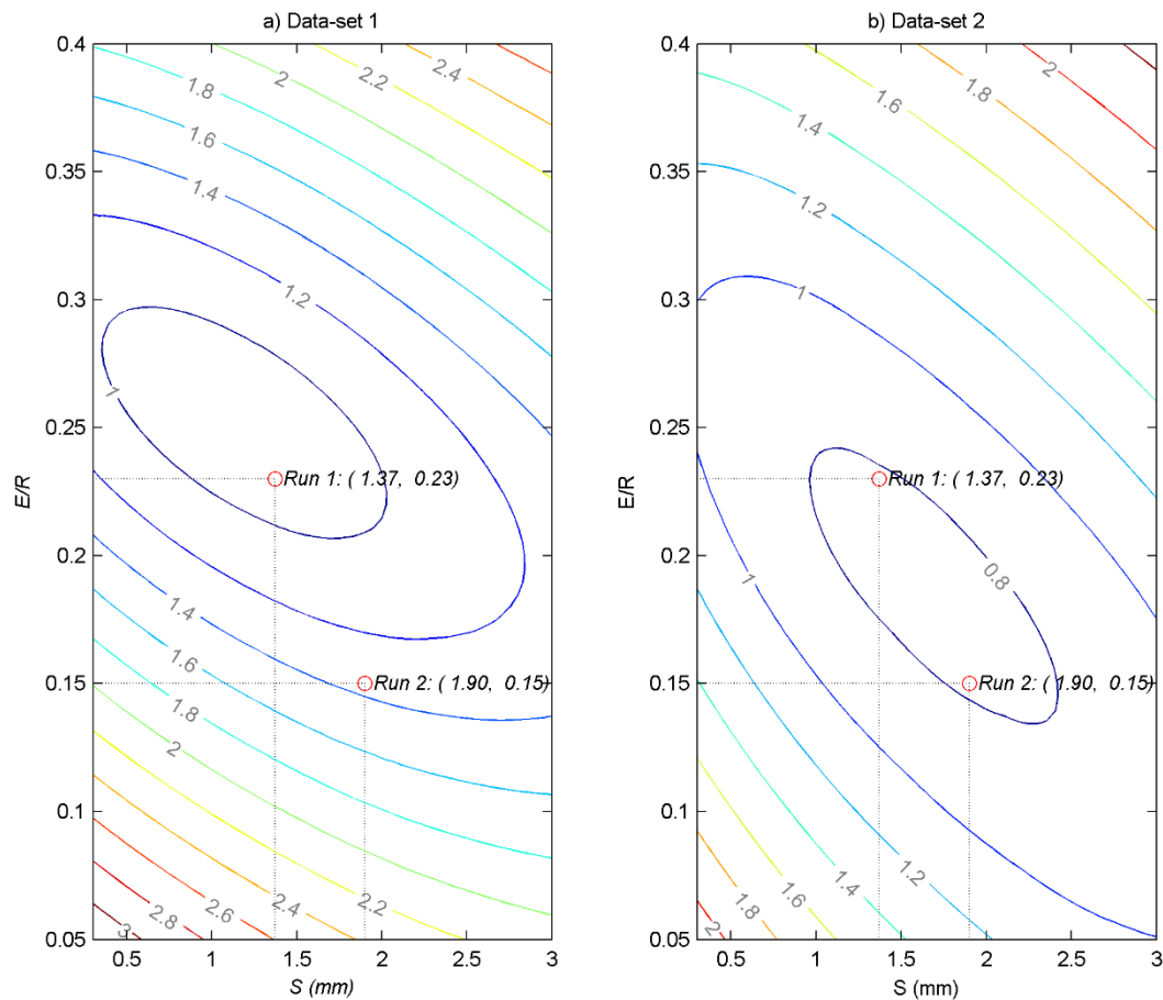
Figure 6. Sensitivity analysis of the parametrized original Gash model. Run 1, all parameters derived from the mean method. Run 2, canopy parameters ( S , \rho ) derived from IEA and E from the energy balance residual method. Contour lines representing the RMSE for different combinations of the parameters' canopy storage capacity ( S ) and the ratio \bar{E}/\bar{R} . (a) Sensitivity analysis using calibration data-set 1 (19 June 2015 to 31 Oct 2015). (b) Sensitivity analysis using validation data-set 2 (19 June 2016 to 31 Oct 2016). The red circles represent the corresponding parameters used in the model Run 1 and Run 2.
