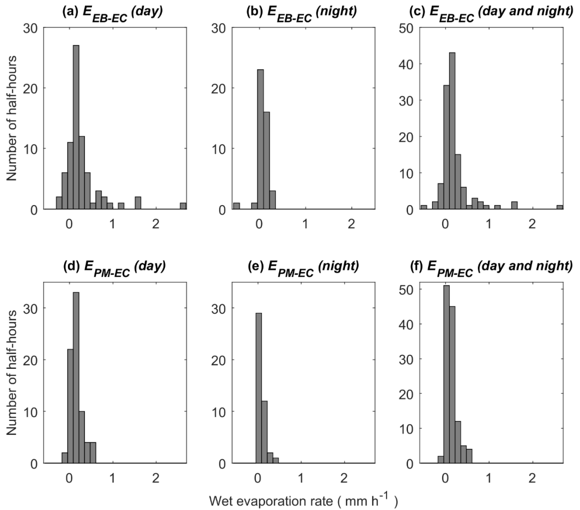
Figure 4. Distributions of wet canopy evaporation rates during day time (7:00-19:00 LT), night time (19:00-7:00 LT) and combined day and night. Two different methods applied: (a-c) energy balance residual ( E_{EB-EC} ) and (d-f) Penman-Monteith ( E_{PM-EC} ).
