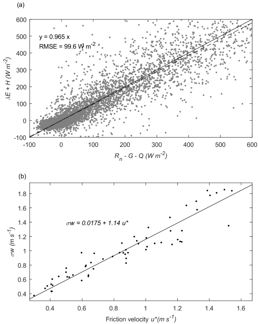
Figure 3. (a) Half-hour interval turbulent heat fluxes ( H and \lambda E ) versus available energy ( R_n - G - Q ) for the study site. Solid line represents 1:1 line and dashed line represents linear regression forced through the origin. (b) Half-hour averages of standard deviation of the vertical wind speed \sigma_w ( m s^{-1} ) versus friction velocity u^* ( m s^{-1} ), wet canopy conditions P_G > 0.5 \text{ mm (30 min)}^{-1} , and near neutral stability ( -0.02 < (z - d)/L < 0.02 ).
